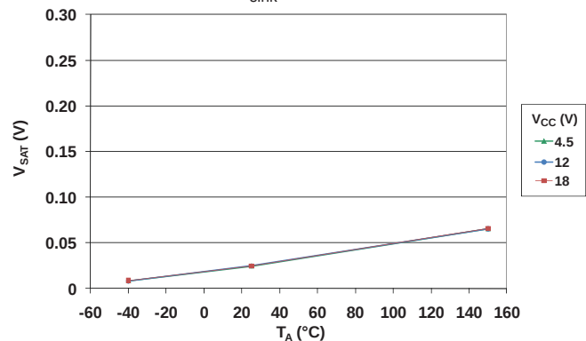
Average PWMOut Saturation Voltage versus Temperature
