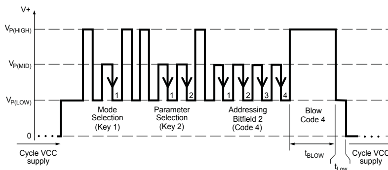
Figure 7. Example of Blow Mode programming pulses applied to the VCC pin. In this example, D_{\text{C(Q)}} (Parameter Key 2) is addressed to code 4 (i.e bit 2) and its value is permanently blown.
