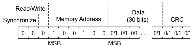
Figure 22. Access Code Write Sequence
