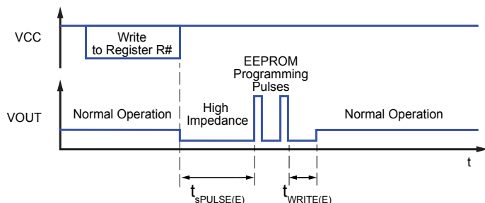
Figure 13. Writing to EEPROM
