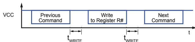
Figure 12. Writing to volatile memory
