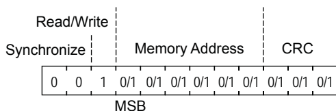
Figure 19. Read Sequence
