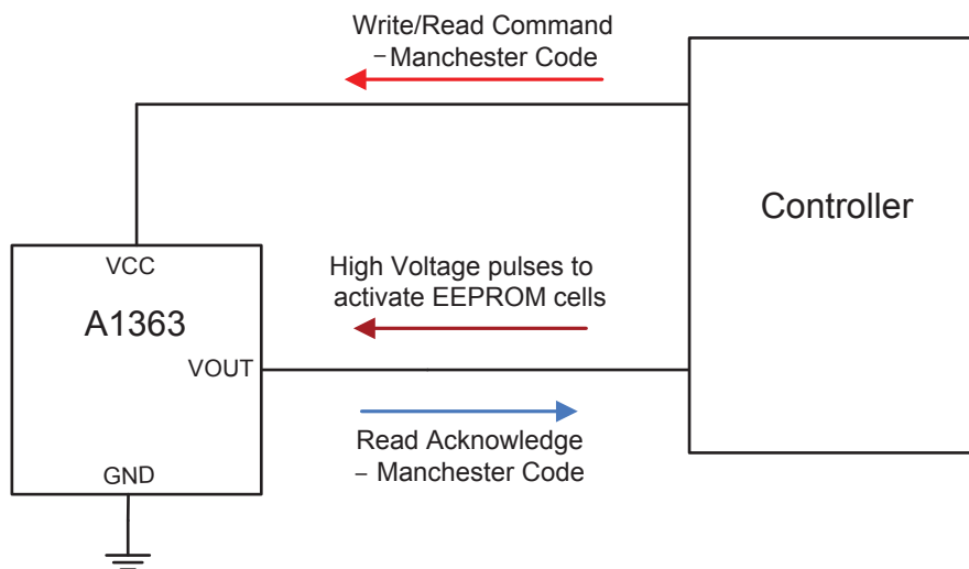
Figure 11. Top level programming interface
