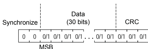
Figure 20. Read Acknowledge Sequence
