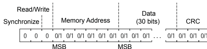
Figure 21. Write Sequence
