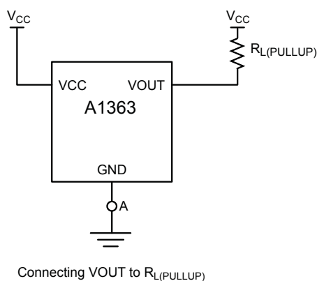
Figure 10. Connections for detecting broken ground wire
