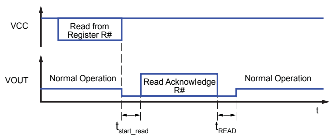
Figure 15. Reading from EEPROM or volatile memory
