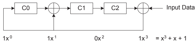
Figure 16. CRC calculation
