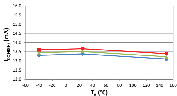
Supply Current (High) versus Ambient Temperature
