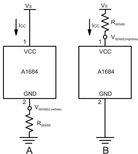
Figure 4: Alternative Polarity Configurations Using Two-Wire Sensing
