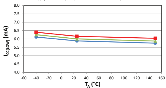
Supply Current (Low) versus Ambient Temperature
