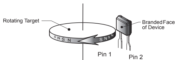
Figure 3: Left-to-Right (pin 1 to pin 2) Direction of Target Rotation.
