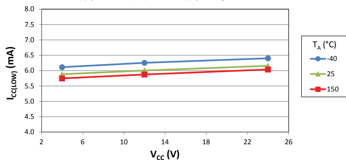
Supply Current (Low) versus Supply Voltage
