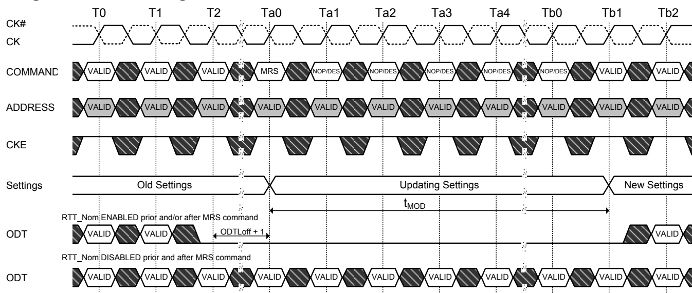
Figure 7. tMOD timing
