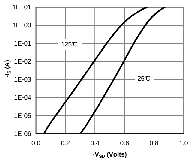
Figure 6: Body-Diode Characteristics
