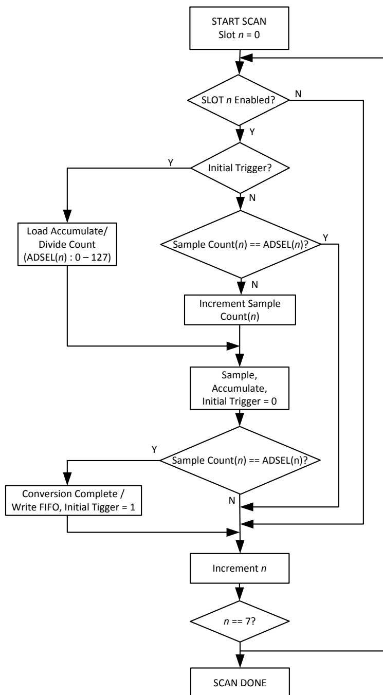
Figure 90. Scan Flowchart
