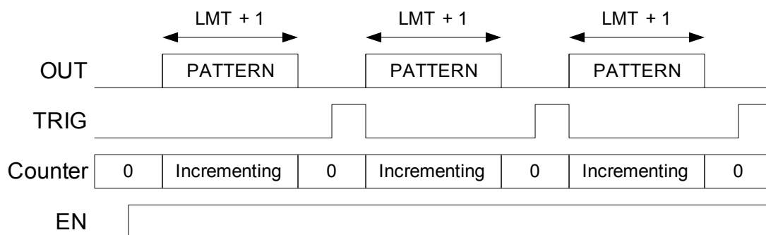
Figure 77. Triggered One-Shot Patterns
