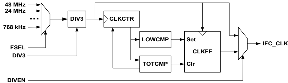
Figure 22. I²C/SPI Master Clock Generation
