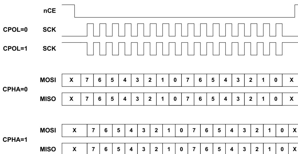
Figure 54. SPI CPOL and CPHA
