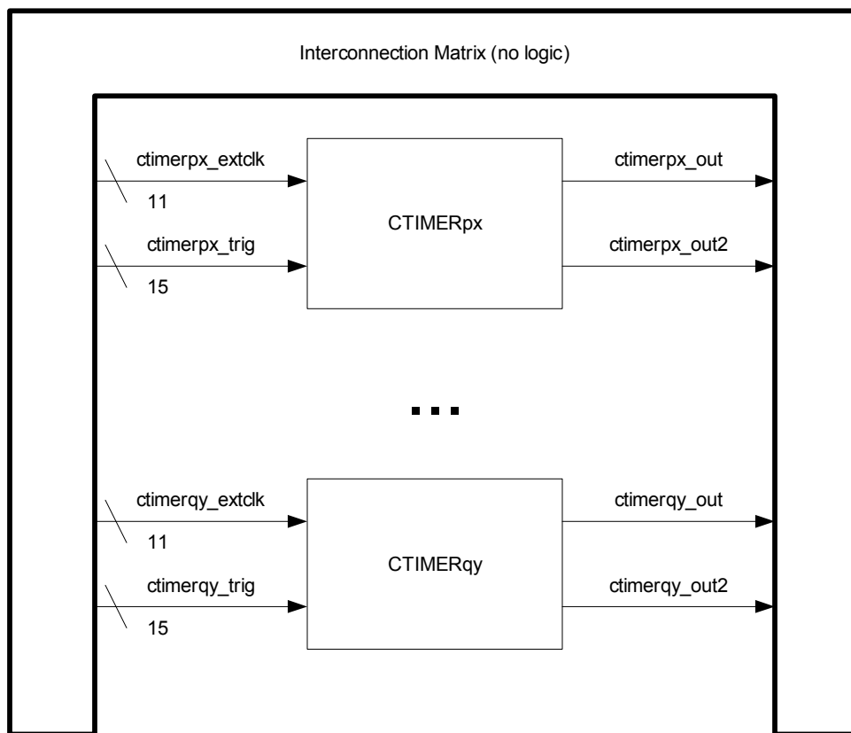
Figure 83. CTIMER Interconnection
