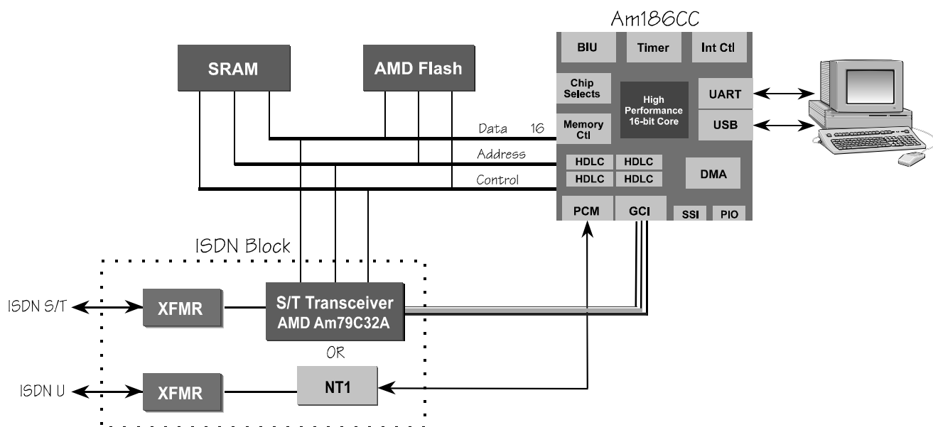
Figure 5. ISDN Terminal Adapter System Application
