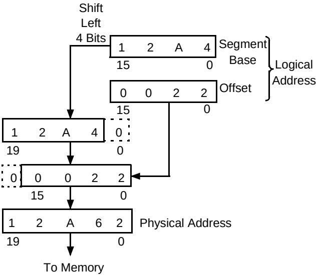
Figure 3. Two-Component Address
