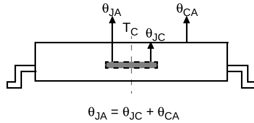
Figure 13. Thermal Resistance (°C/Watt)
