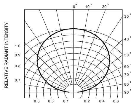
RADIATION DIAGRAM
