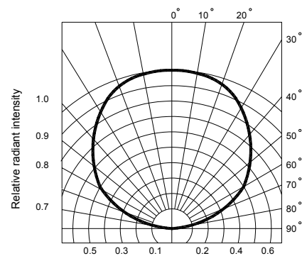
Fig.6 Radiation diagram
