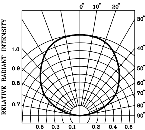
Fig.6 RADIATION DIAGRAM
