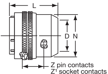
“SP”, MS / “P” 灌封套管
