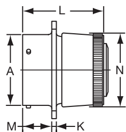
MF00SE-XX-XXX MS3128E-XX-XXX
