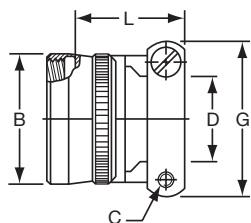
等级“A”&“P”抗拉力电缆夹 10-101980-XX
