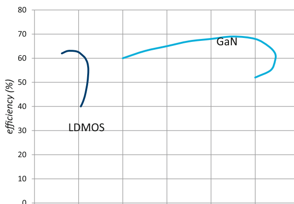
GaN vs LDMOS Comparison @ 2.1 GHz
