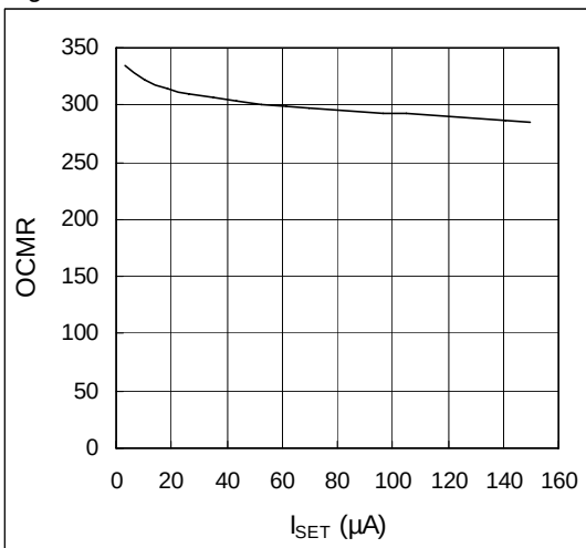
Figure 8. AS1102, AS1103, AS1104 OMCR vs. I_{SET}
