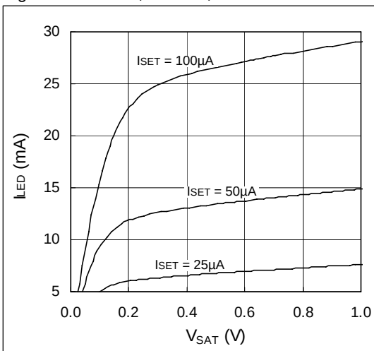
Figure 6. AS1102, AS1103, AS1104 I_{LED} vs. V_{SAT}
