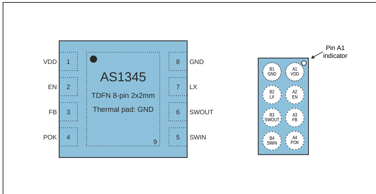
Figure AS1345 – 4: Pin Assignments (Top View)
