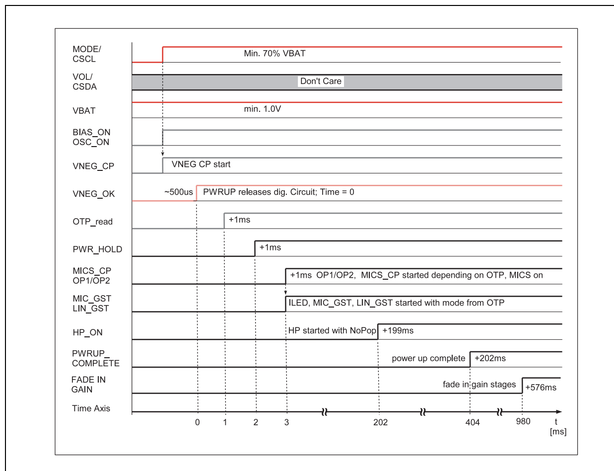
Figure 51: Start-Up Sequence
