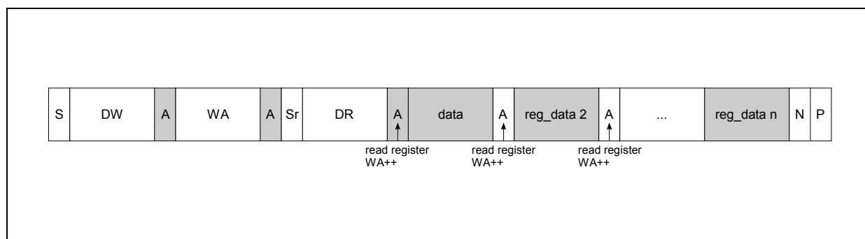
Figure 80: Sequential Read
