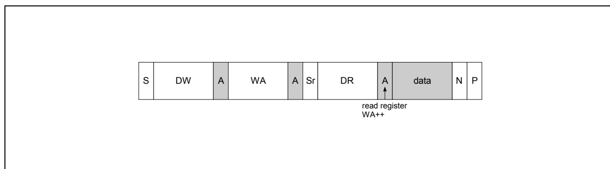
Figure 79: Random Read
