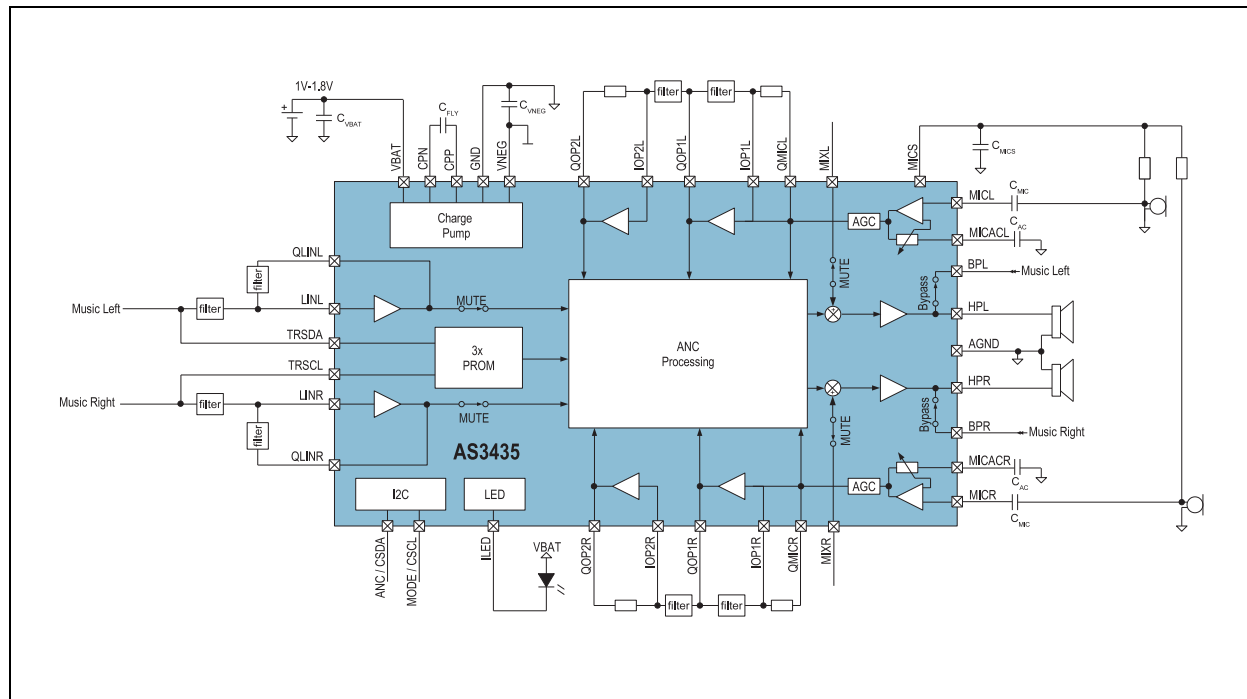
Figure 3: AS3435 Block Diagram
