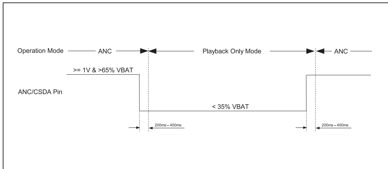
Figure 60: Playback Only Mode Timing Diagram
