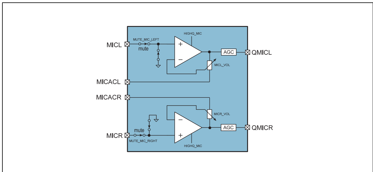
Figure 19: Stereo Microphone Input
