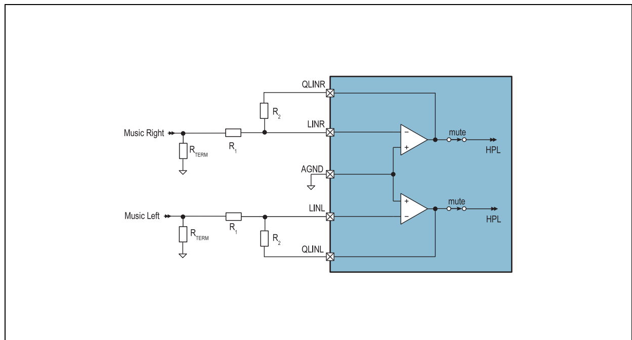
Figure 8: Stereo Line Input
