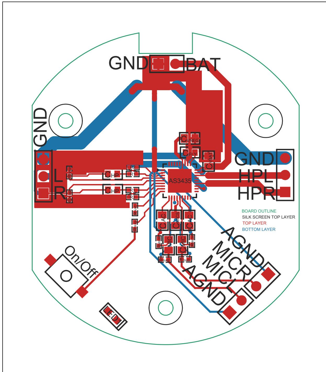
Figure 110: AS3435 Over the Ear Layout Example
