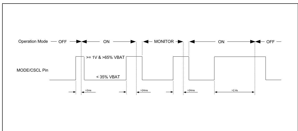
Figure 59: Push Button Mode Timing Diagram
