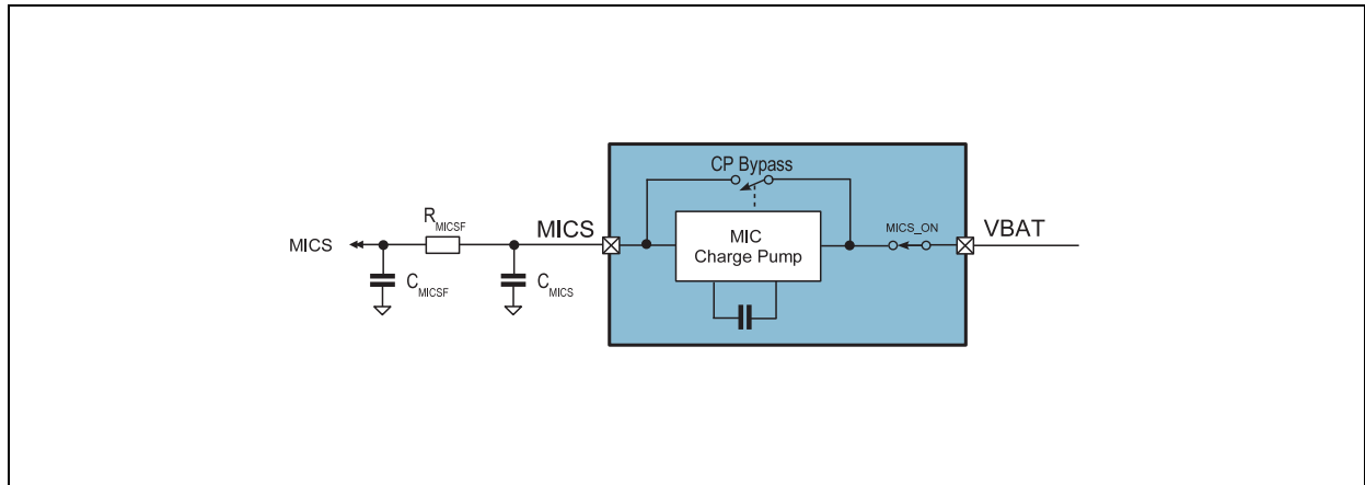
Figure 27: Microphone Supply
