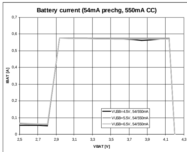
Figure 7. Charging Cycle 1
