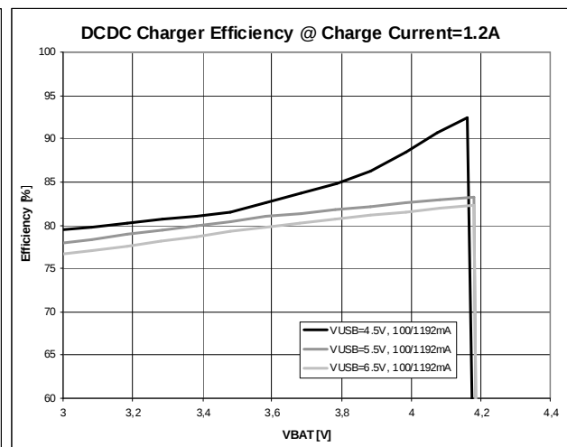
Figure 10. Efficiency @1.2A
