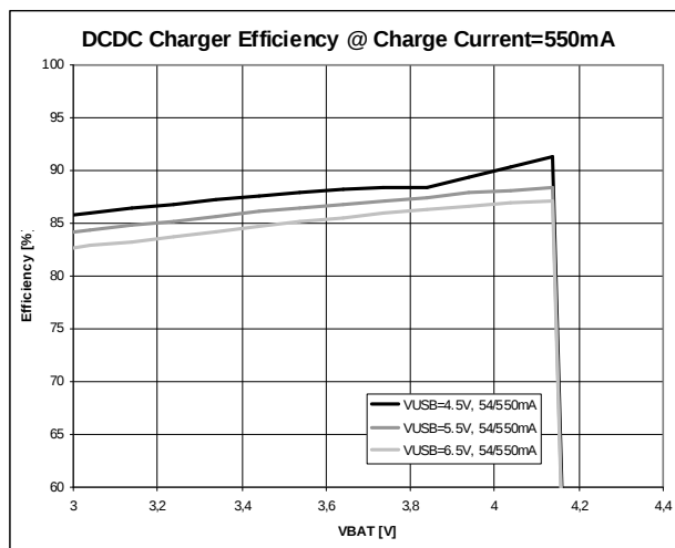
Figure 9. Efficiency @550mA
