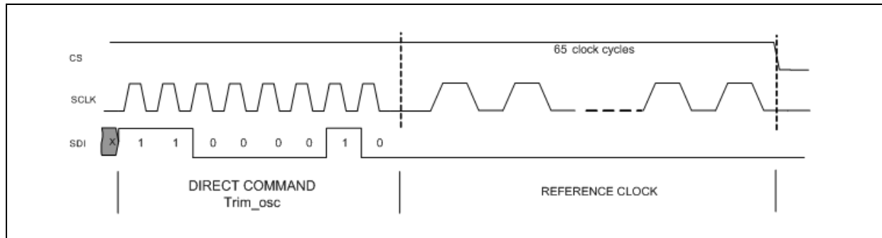
Figure 19. RC-Oscillator calibration via SDI
