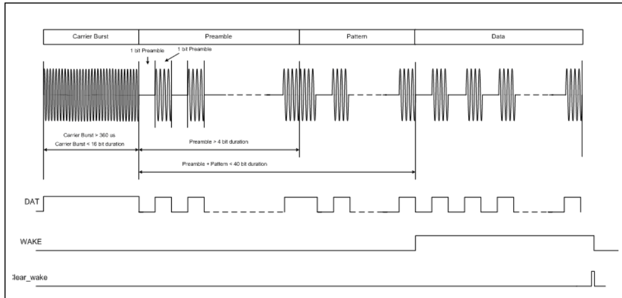
Figure 17. Wakeup protocol overview with single pattern detection
