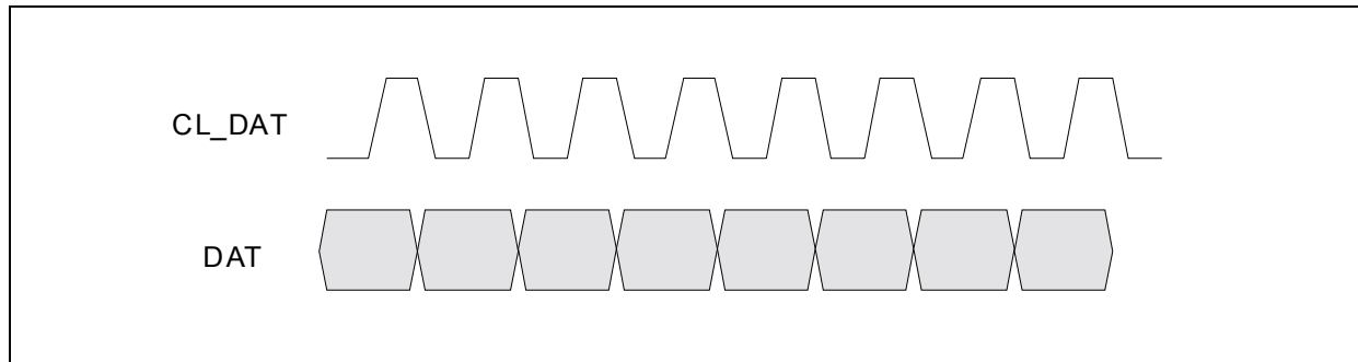
Figure 15. Synchronisation of data with recovered Manchester clock
