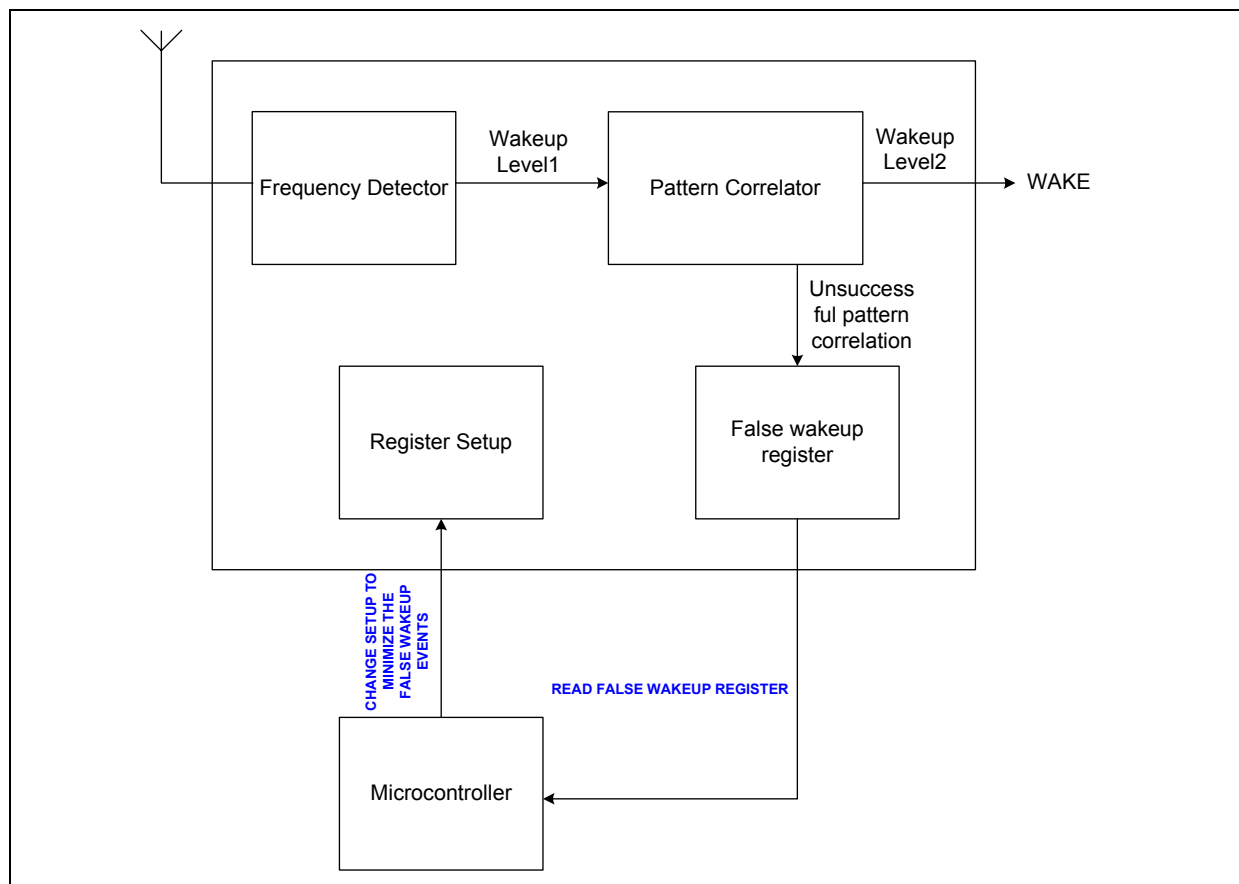
Figure 18. Concept of the false wakeup register together with the system.
