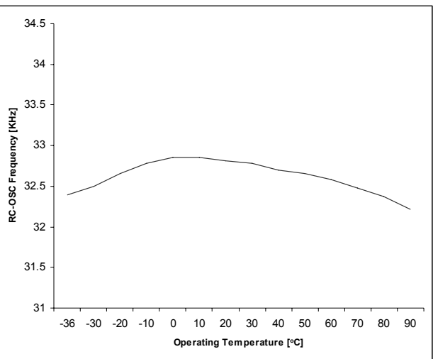
Figure 7. RC-Osc Frequency over Temperature (calibr.)
