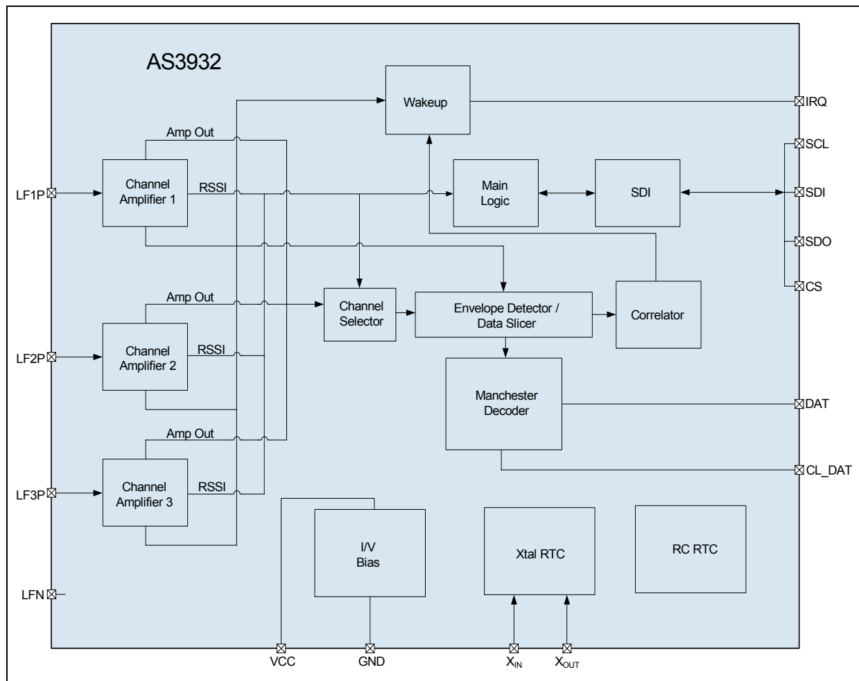
Figure 8. Block Diagram
