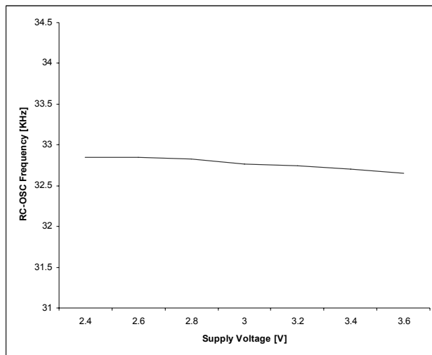
Figure 6. RC-Osc Frequency over Voltage (calibr.)
