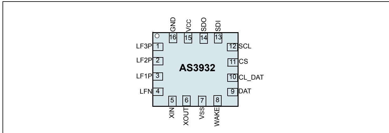
Figure 3. Pin Assignments QFN 4x4 16LD Package
