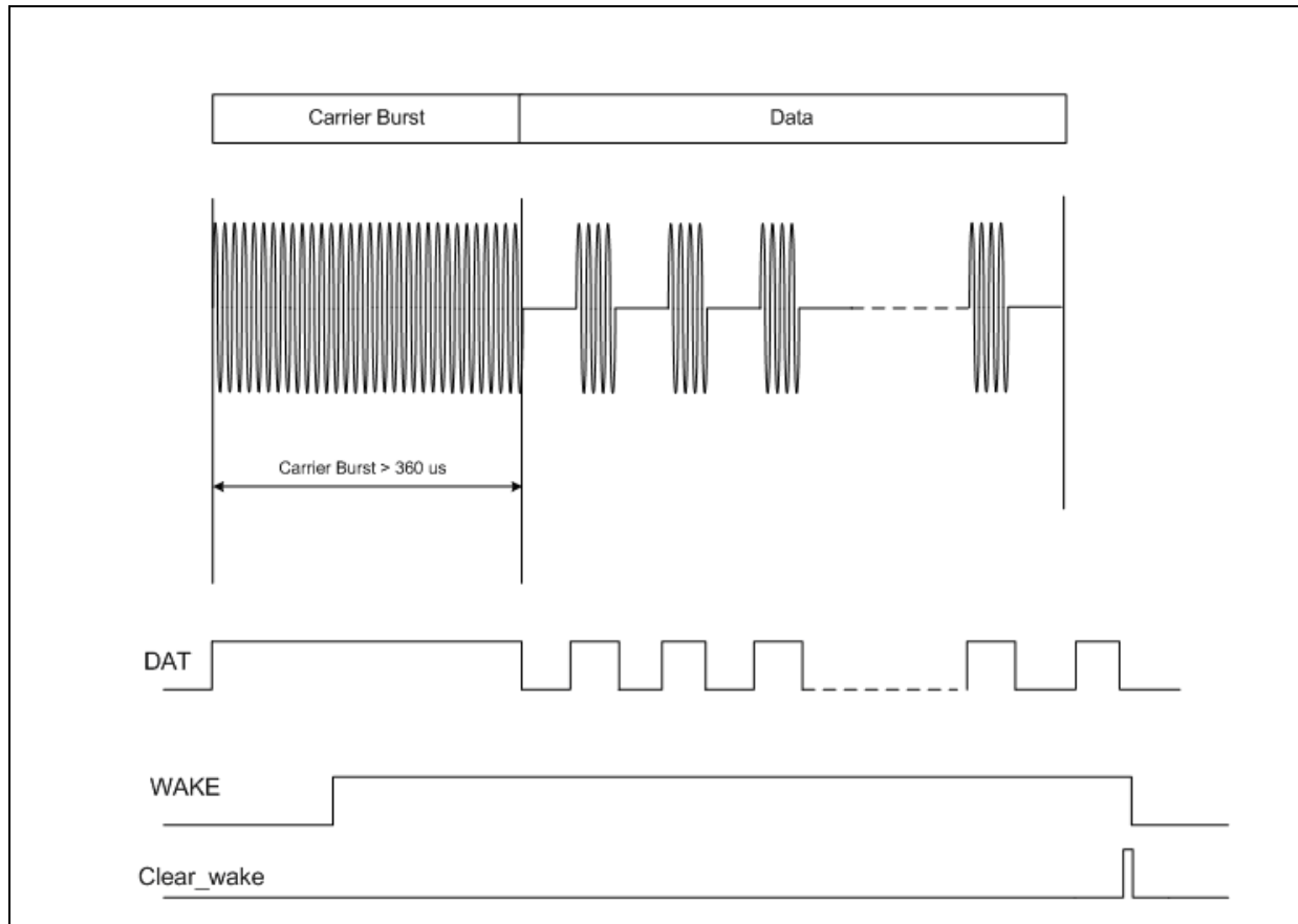
Figure 16. Wakeup protocol overview without pattern detection (only carrier frequency detection)
