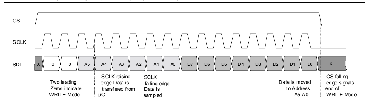
Figure 12. Writing of Register Data with auto-incrementing Address
