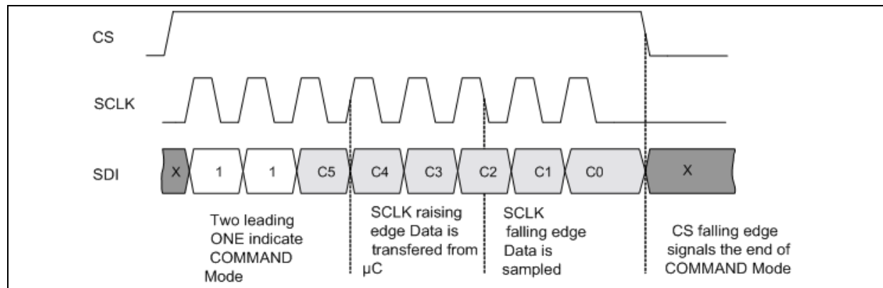
Figure 14. Send direct COMMAND byte
