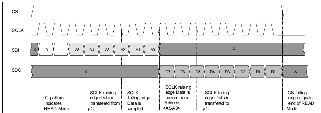
Figure 13. Reading of a single Register Byte
