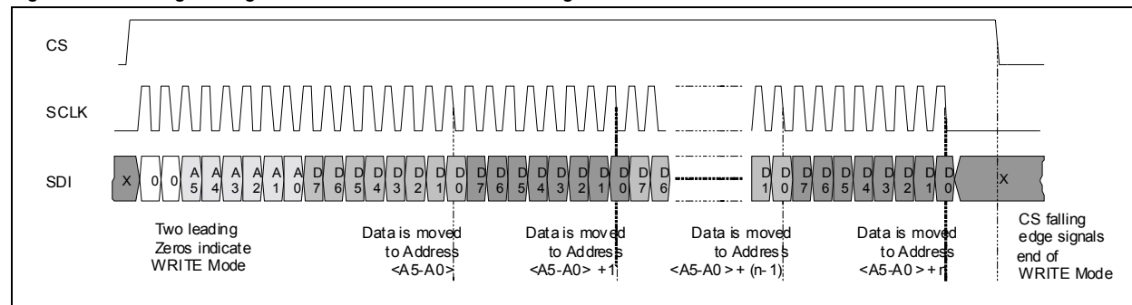
Figure 12. Writing of Register Data with auto-incrementing Address
