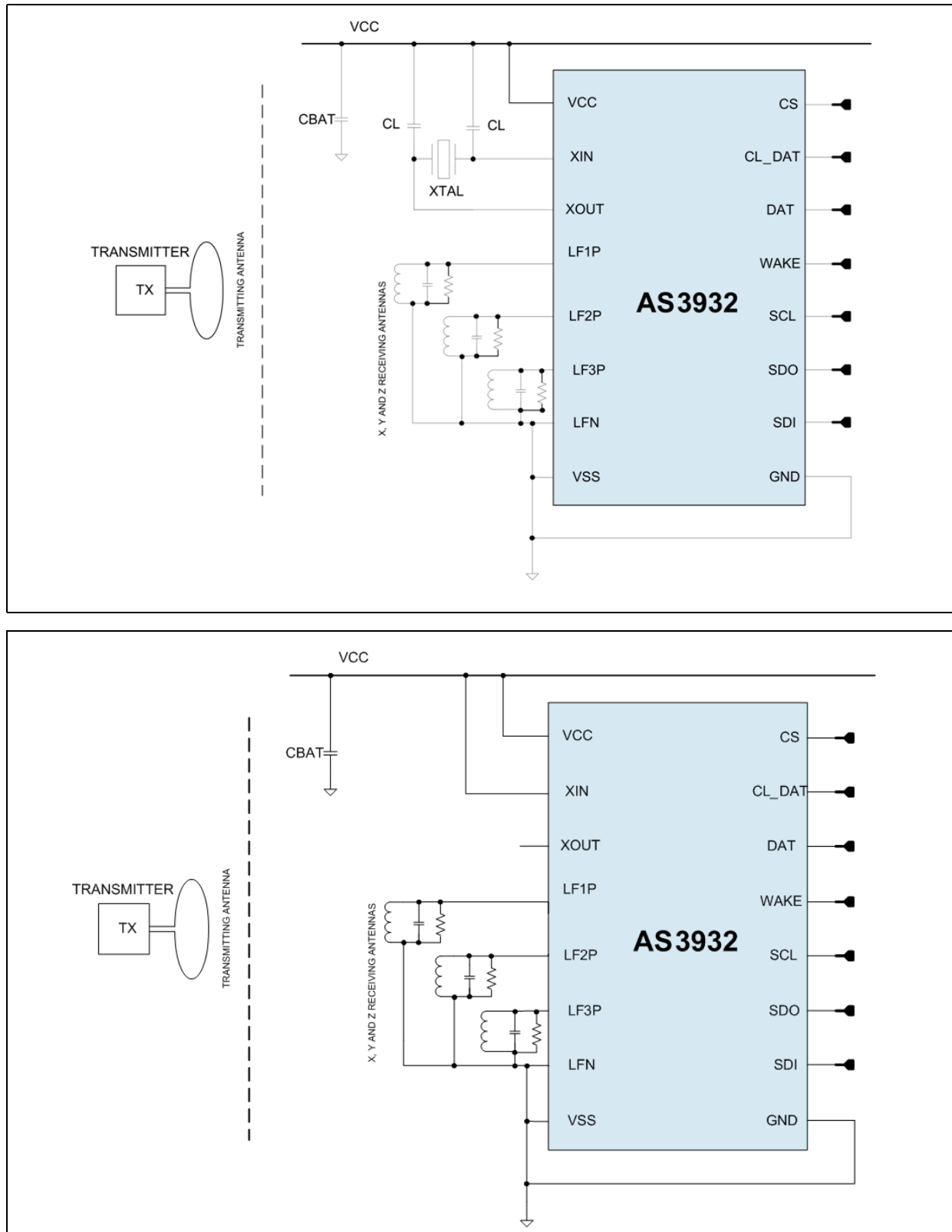
Figure 1. Typical Application Diagrams with crystal (top) and without crystal (bottom)
