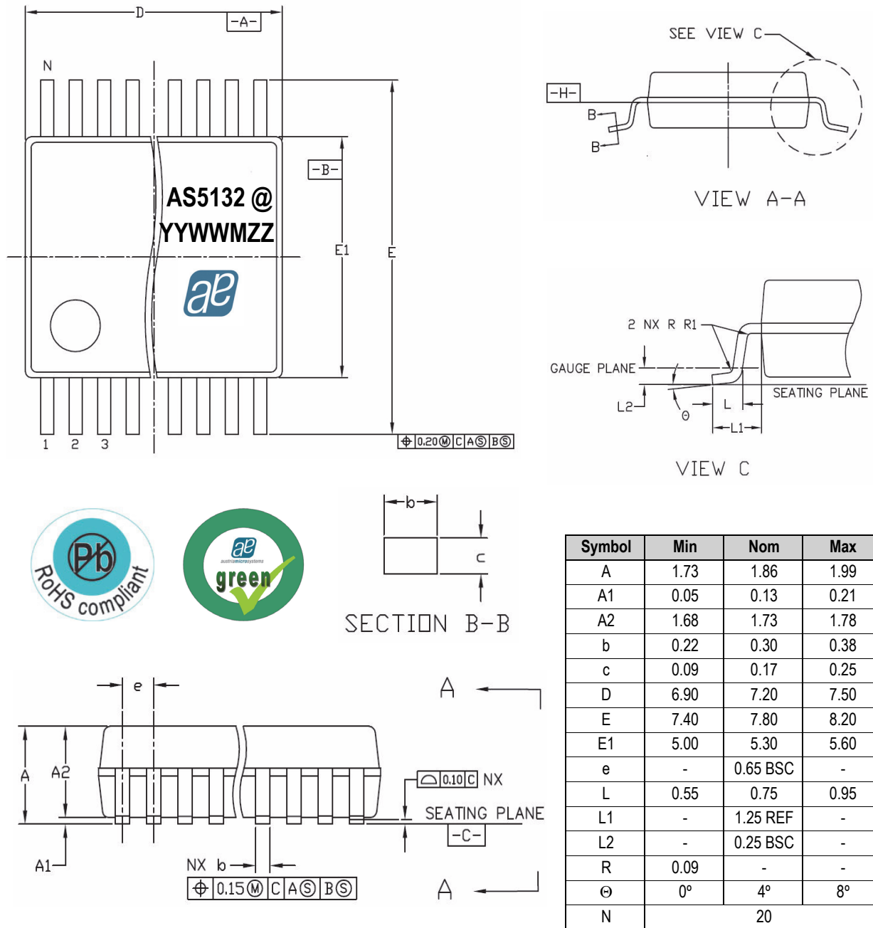
Figure 24. Package Drawings and Dimensions
