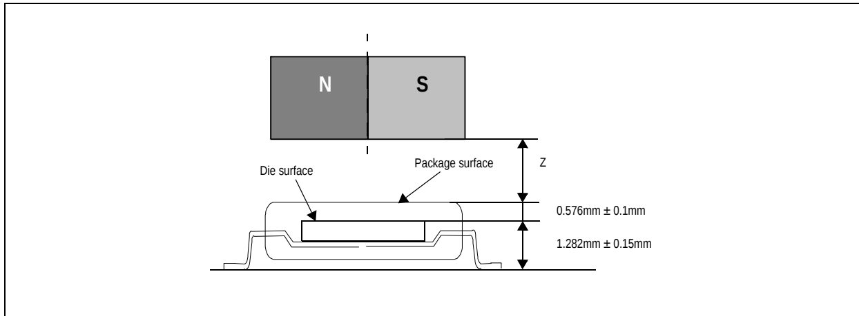
Figure 20. Vertical Placement of the Magnet
