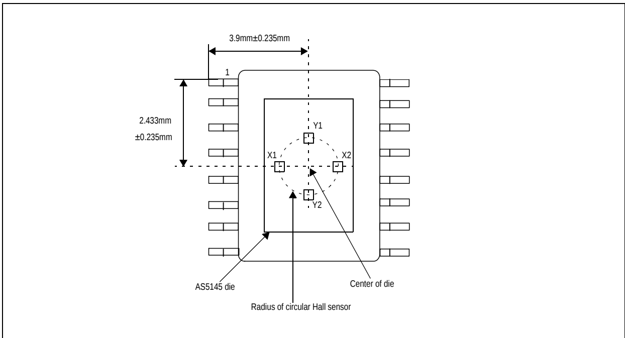
Figure 21. Arrangement of Hall Sensor Array on Chip (principle)
