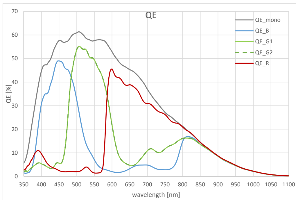
Figure 8 : Quantum Efficiency
