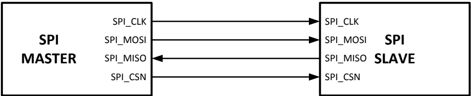
Figure 21: SPI Connection Diagram
