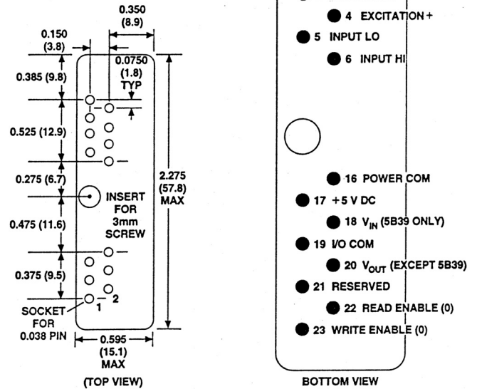
Figure 4 . Model 5B Series Module, with pin-out assignments.
