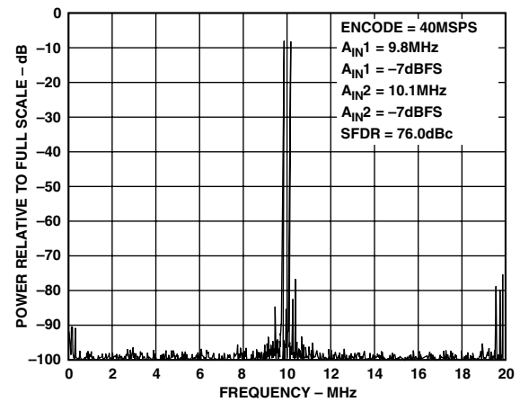
TPC 4. Two-Tone FFT @ 9.8 MHz/10.1 MHz
