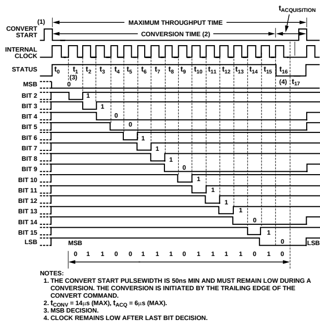
Figure 6. Timing Diagram (Binary Code 0110011101111010)
