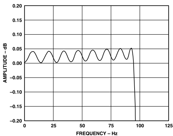
TPC 9. AD1556 Pass Band Ripple, F_O = 250 Hz (4 ms)
