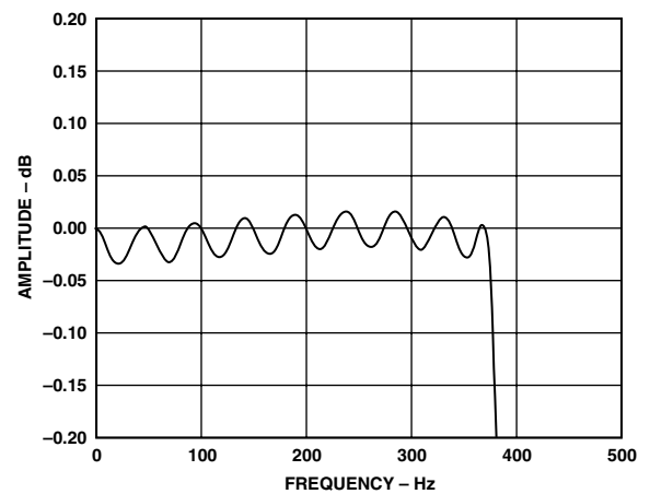
TPC 11. AD1556 Pass Band Ripple, F_O = 1 kHz (1 ms)
