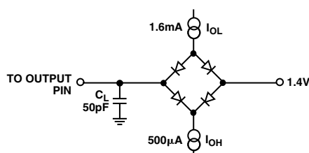
Figure 2. Load Circuit for Digital Interface Timing
