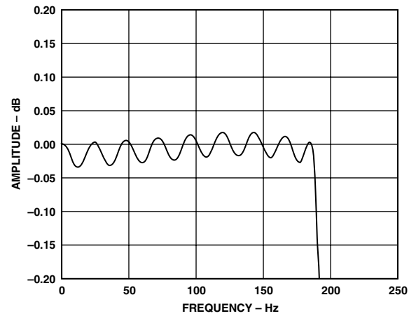
TPC 10. AD1556 Pass Band Ripple, F_O = 500 Hz (2 ms)
