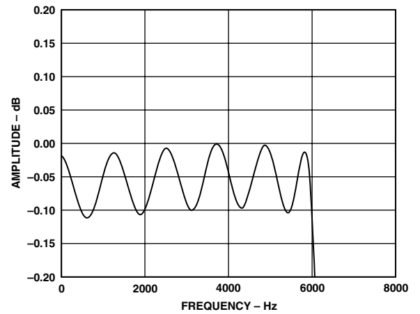
TPC 15. AD1556 Pass Band Ripple, F_O = 16 \text{ kHz} (1/16 ms)
