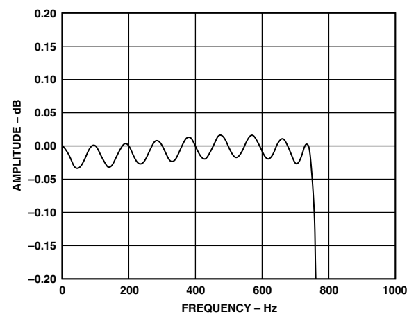
TPC 12. AD1556 Pass Band Ripple, F_O = 2 kHz (1/2 ms)
