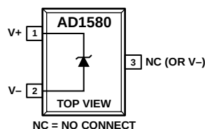
Figure 1. SOT-23
