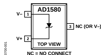
Figure 2. SC70
