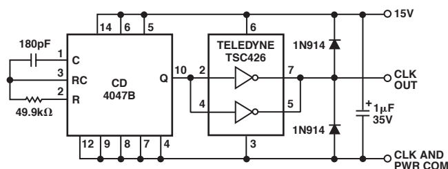
Figure 4. Clock Driver
