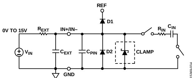
Figure 43. Equivalent Analog Input Circuit
