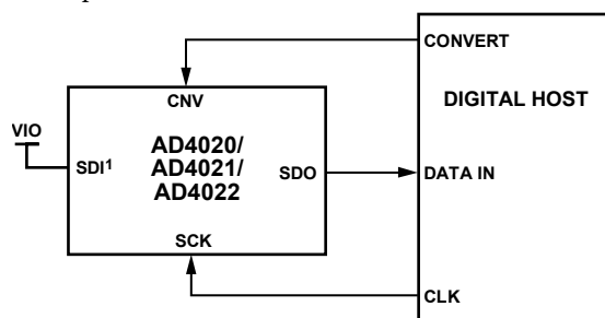
Figure 55. \overline{CS} Mode, 3-Wire Without Busy Indicator Connection Diagram
