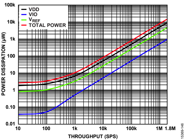
Figure 35. Power Dissipation vs. Throughput, V_{IO} = 1.8\text{ V} , V_{REF} = 5\text{ V}
