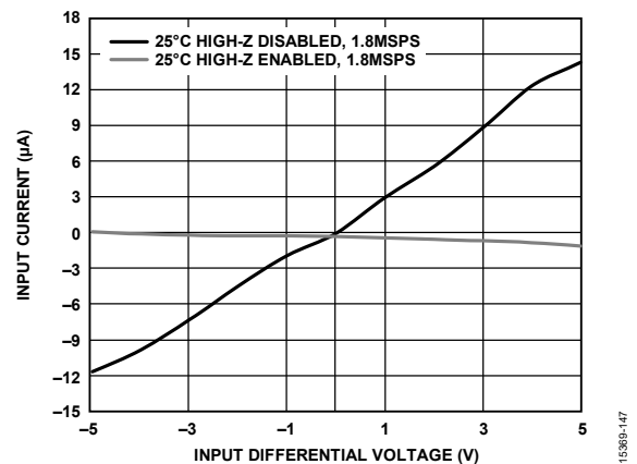
Figure 2. Input Current vs. Input Differential Voltage
