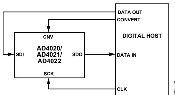
Figure 53. \overline{CS} Mode, 3-Wire Turbo Mode Connection Diagram
