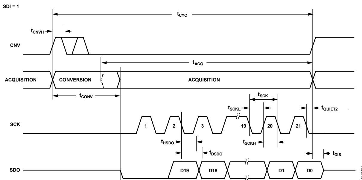
Figure 58. \overline{\text{CS}} Mode, 3-Wire with the Busy Indicator Serial Interface Timing Diagram (Status Bits Not Shown)
