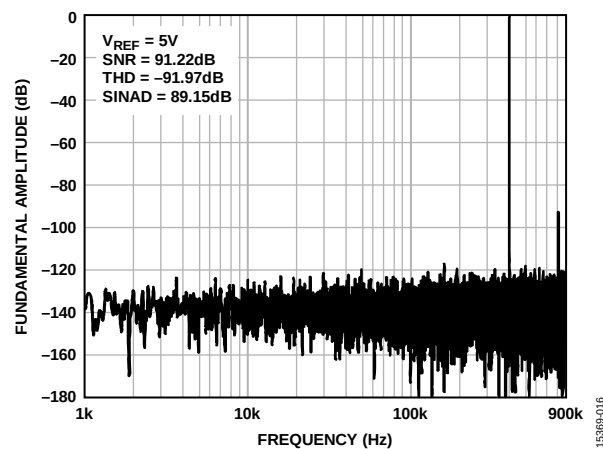
Figure 16. 400 kHz, -0.5 dBFS Input Tone FFT
