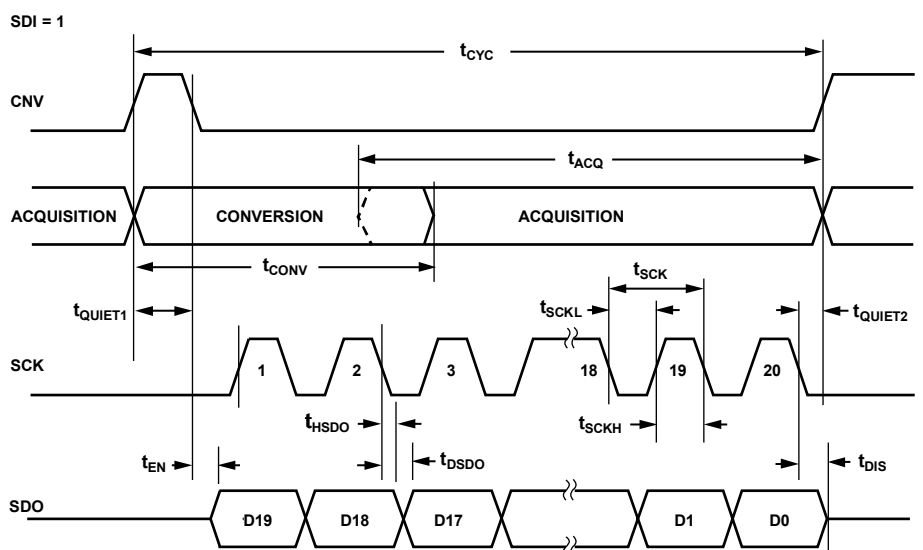
Figure 54. \overline{CS} Mode, 3-Wire Turbo Mode Serial Interface Timing Diagram (Status Bits Not Shown)
