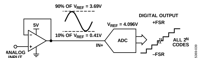
Figure 46. Span Compression
