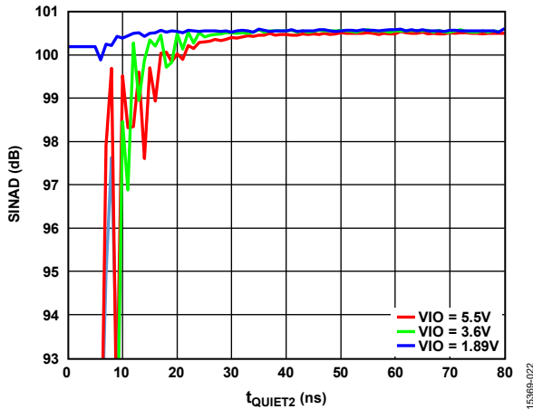
Figure 24. SINAD vs. t_{\text{QUIET2}}
