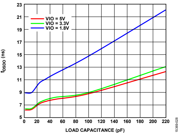
Figure 37. t_{DSO} vs. Load Capacitance
