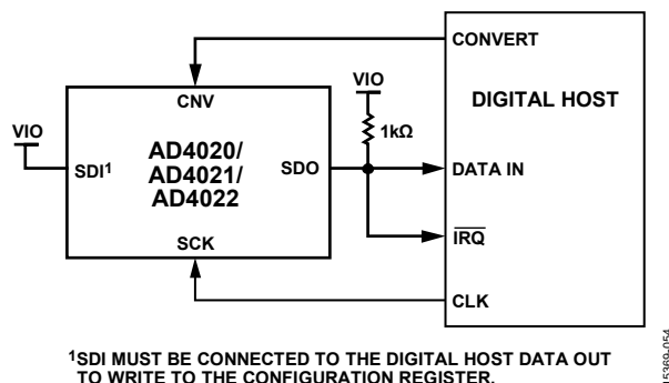
Figure 57. \overline{\text{CS}} Mode, 3-Wire with Busy Indicator Connection Diagram
