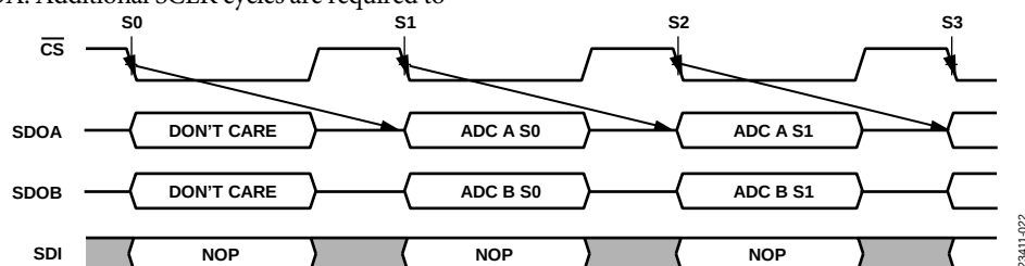
Figure 41. Reading Conversion Results: 2-Wire Mode
