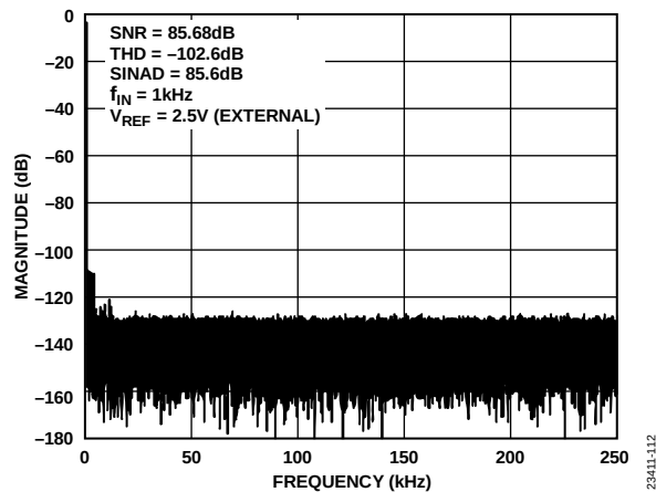
Figure 11. AD4683 FFT, V_{REF} = 2.5\text{ V} External
