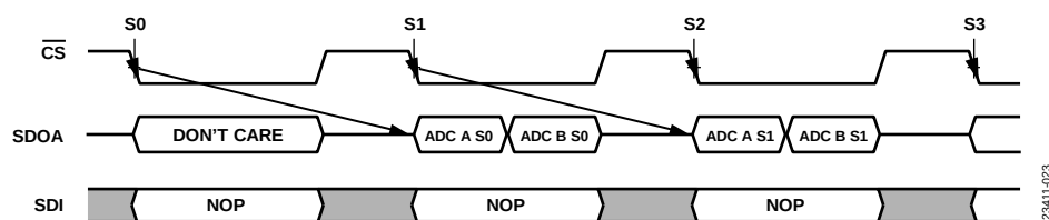
Figure 42. Reading Conversion Results: 1-Wire Mode
