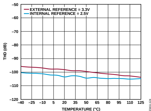
Figure 23. AD4682 THD vs. Temperature
