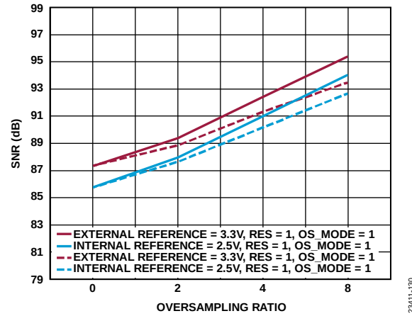
Figure 29. AD4682 SNR vs. Oversampling Ratio, Rolling Average Oversampling
