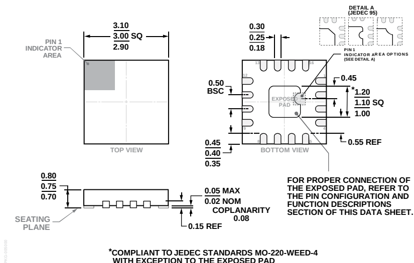
Figure 47. 16-Lead Lead Frame Chip Scale Package [LFCSP] 3 mm × 3 mm Body and 0.75 mm Package Height (CP-16-45) Dimensions shown in millimeters
