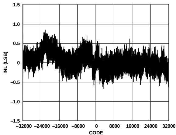
Figure 13. Typical INL Error
