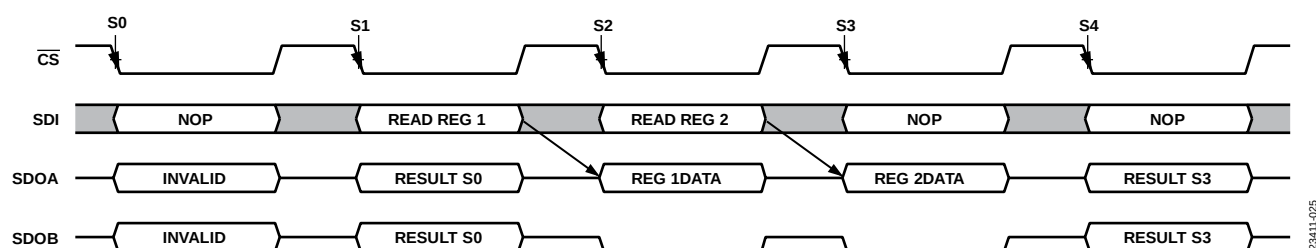
Figure 44. Register Read
