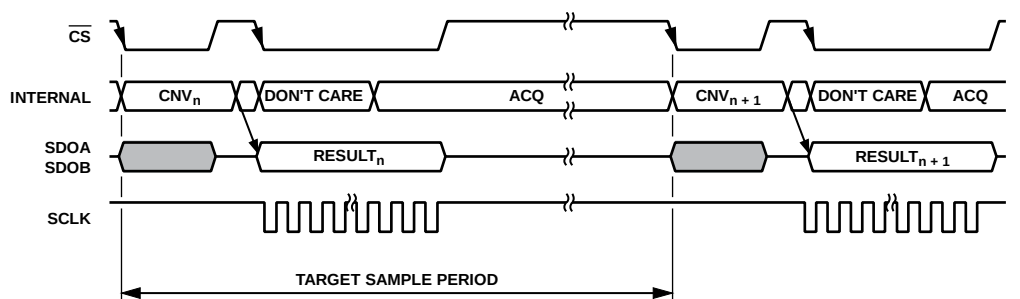
Figure 43. Low Throughput Low Latency
