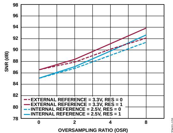
Figure 30. AD4683 SNR vs. Oversampling Ratio, Rolling Average Oversampling
