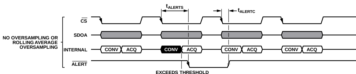
Figure 37. Alert Operation
