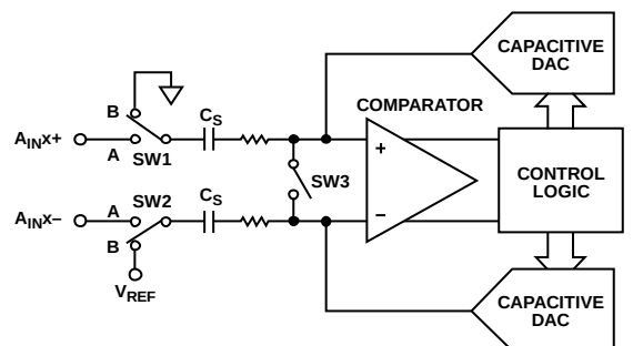
Figure 32. ADC Conversion Phase
