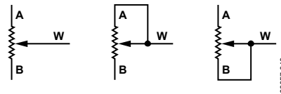
Figure 42. Rheostat Mode Configuration
