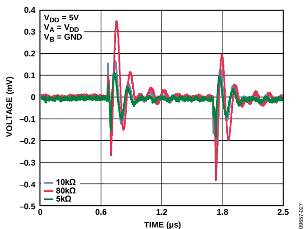
Figure 27. Digital Feedthrough
