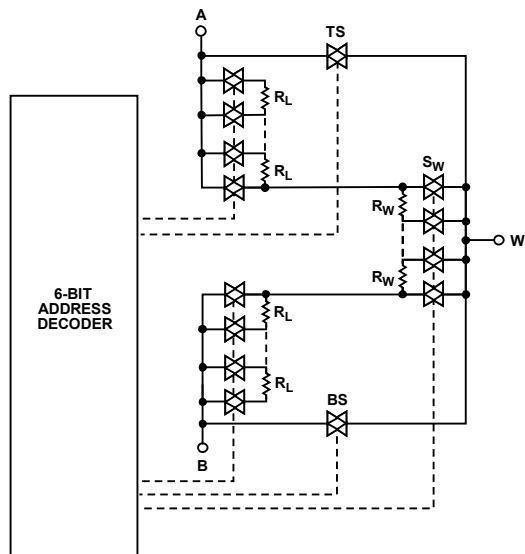
Figure 41. Simplified RDAC Circuit
