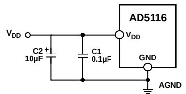
Figure 45. Power Supply Bypassing
