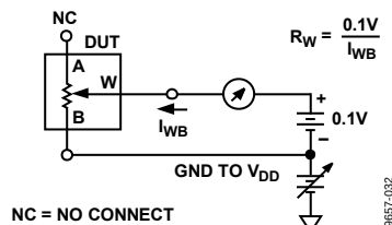
Figure 34. Wiper Resistance
