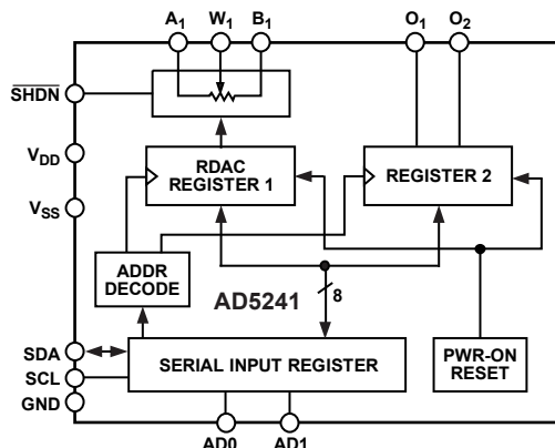
Figure 1. AD5241 Functional Block Diagram
