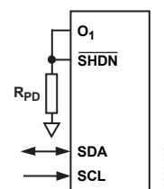
Figure 35. Shutdown by Internal Logic Output, O_1
