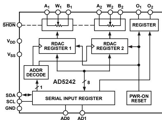
Figure 2. AD5242 Functional Block Diagram
