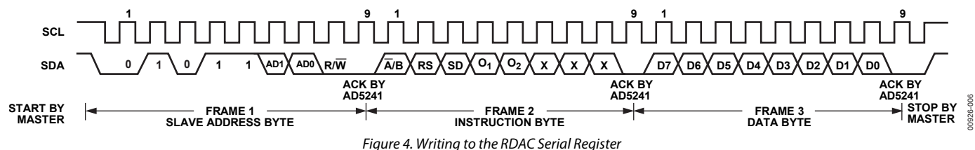
Figure 4. Writing to the RDAC Serial Register
