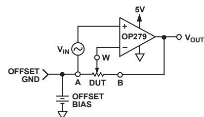
Figure 27. Noninverting Gain
