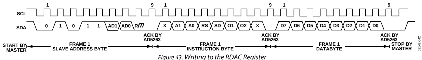
Figure 43. Writing to the RDAC Register
