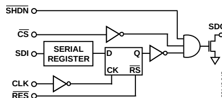
Figure 46. Detailed SDO Output Schematic of the AD5263
