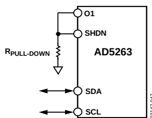
Figure 48. Shutdown by Internal Logic Output
