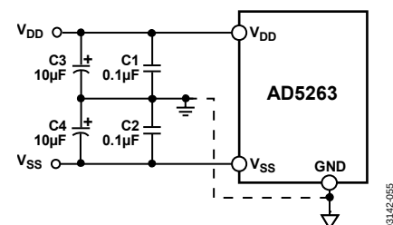
Figure 55. Power Supply Bypassing
