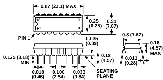
16-Lead Plastic DIP Package (N-16)
