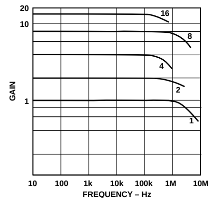
Figure 6. Gain vs. Frequency
