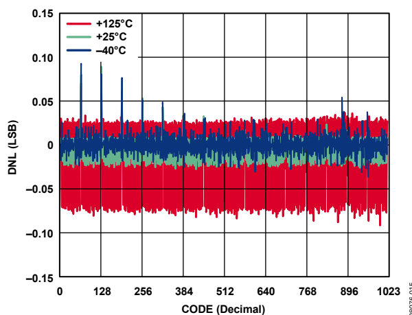
Figure 9. R-DNL in Normal Mode vs. Code vs. Temperature (AD5272)
