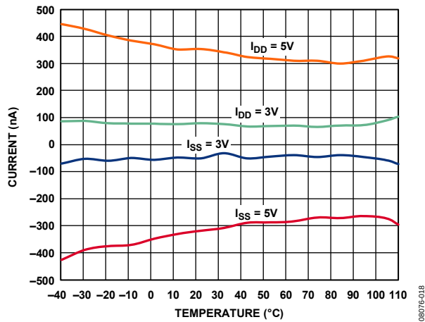
Figure 12. Supply Current ( I_{DD} , I_{SS} ) vs. Temperature
