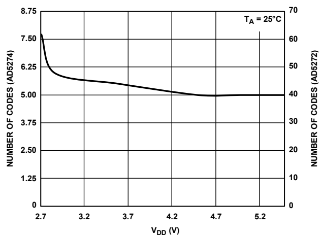
Figure 21. Maximum Code Loss vs. Power Supply Range
