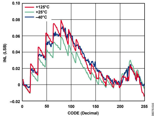
Figure 11. R-INL in Normal Mode vs. Code vs. Temperature (AD5274)
