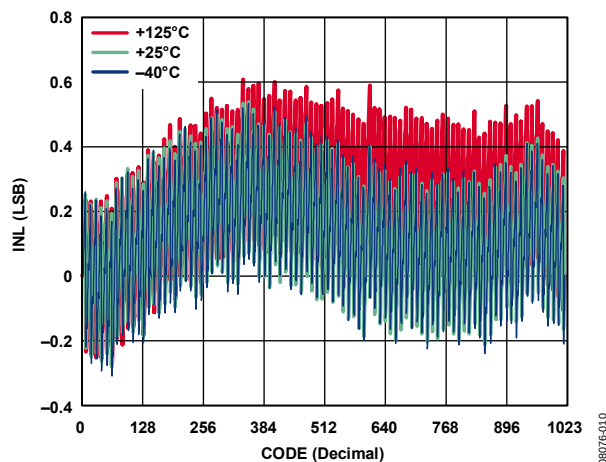
Figure 5. R-INL in R-Perf Mode vs. Code vs. Temperature (AD5272)
