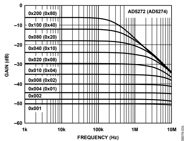
Figure 16. Bandwidth vs. Code vs. Frequency
