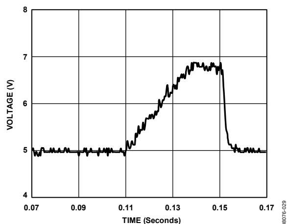
Figure 22. V_{EXT\_CAP} Waveform While Writing Fuse
