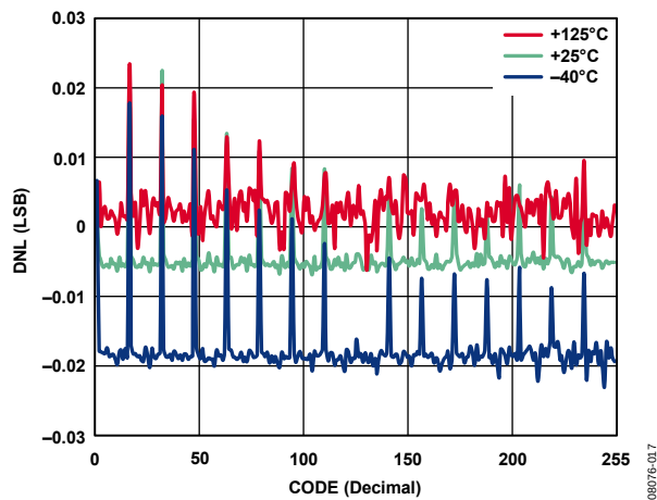
Figure 13. R-DNL in Normal Mode vs. Code vs. Temperature (AD5274)
