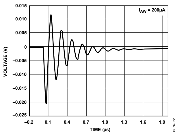
Figure 23. Maximum Glitch Energy
