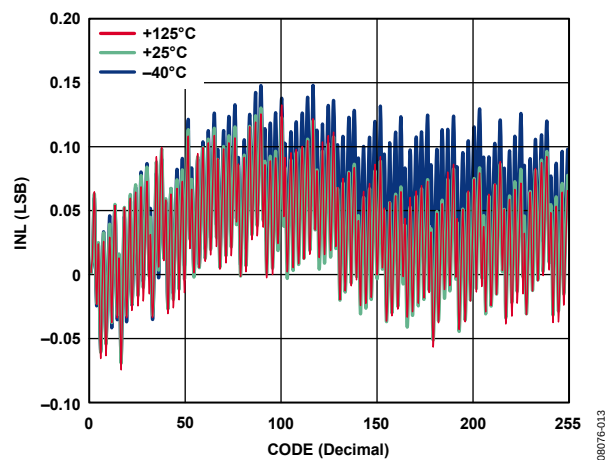
Figure 7. R-INL in R-Perf Mode vs. Code vs. Temperature (AD5274)
