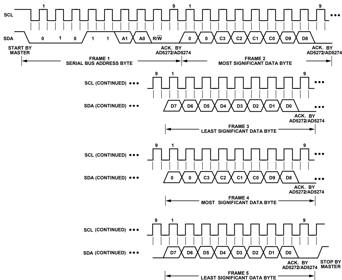
Figure 30. Multiple Write
