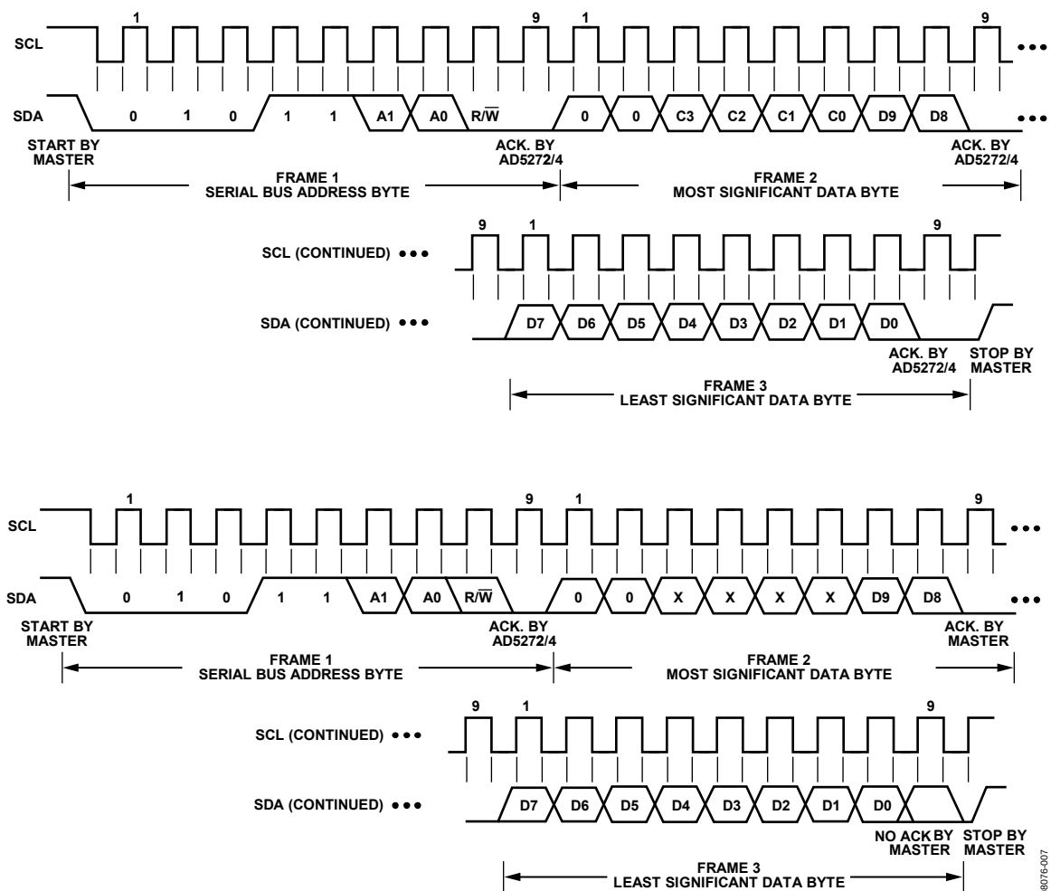
Figure 31. Read Command
