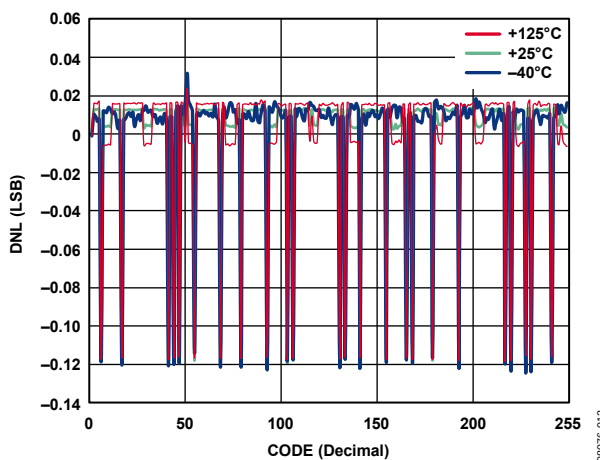
Figure 10. R-DNL in R-Perf Mode vs. Code vs. Temperature (AD5274)
