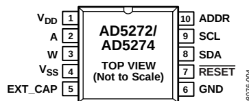
Figure 4. Pin Configuration
