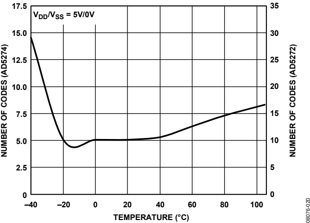
Figure 18. Maximum Code Loss vs. Temperature
