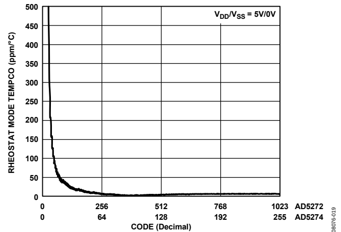
Figure 14. Tempco \Delta R_{WA}/\Delta T vs. Code
