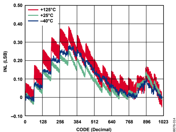
Figure 6. R-INL in Normal Mode vs. Code vs. Temperature (AD5272)
