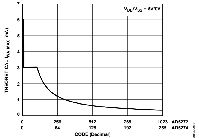
Figure 15. Theoretical Maximum Current vs. Code
