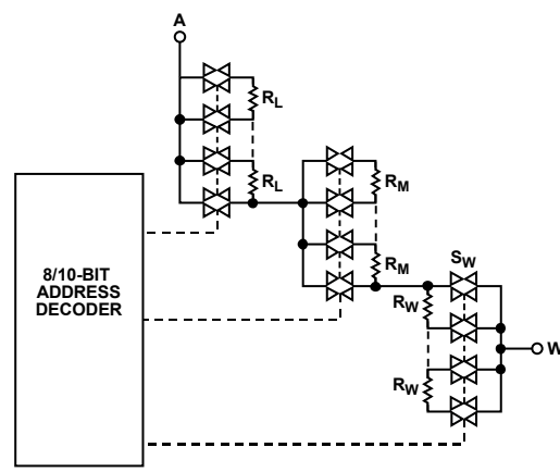
Figure 32. Simplified RDAC Circuit
