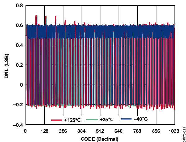
Figure 8. R-DNL in R-Perf Mode vs. Code vs. Temperature (AD5272)
