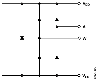
Figure 34. Maximum Terminal Voltages Set by V_{DD} and V_{SS}
