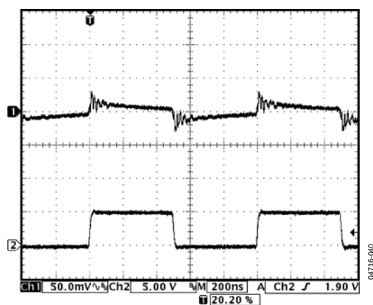
Figure 24. Digital Feedthrough
