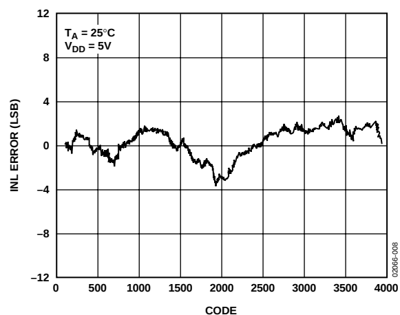
Figure 8. AD5326 Typical INL Plot
