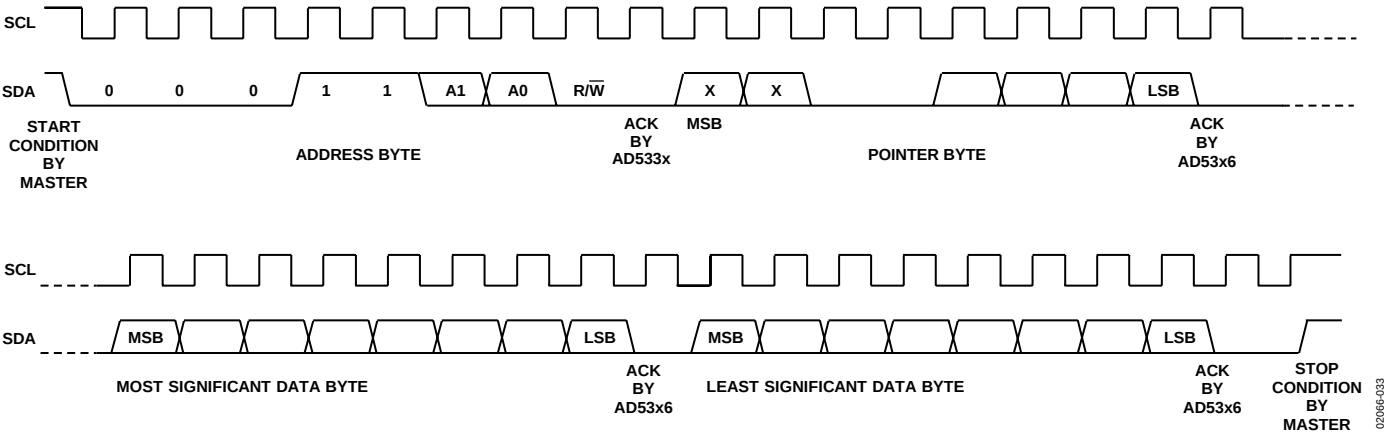
Figure 33. Write Sequence
