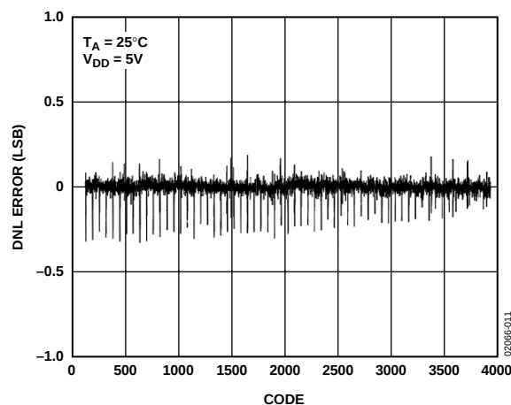
Figure 11. AD5326 Typical DNL Plot
