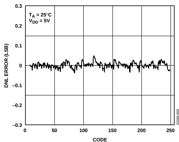
Figure 9. AD5306 Typical DNL Plot
