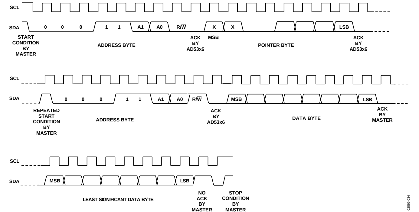
Figure 34. Readback Sequence
