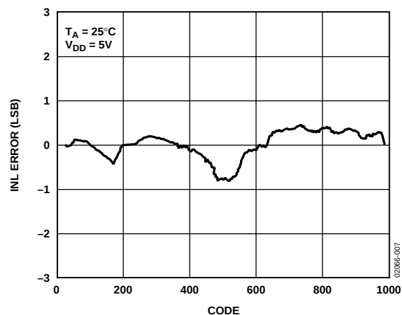
Figure 7. AD5316 Typical INL Plot
