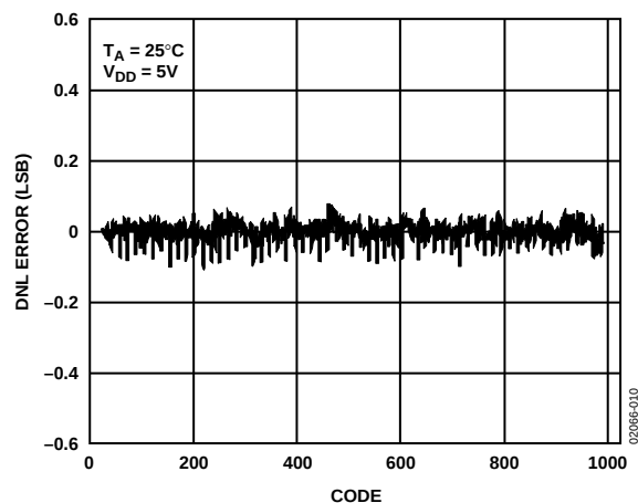
Figure 10. AD5316 Typical DNL Plot
