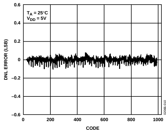
Figure 10. AD5316 DNL
