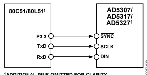
Figure 39. 80C51/80L51-to-AD5307/AD5317/AD5327 Interface
