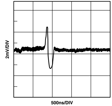
TPC 21. DAC-DAC Crosstalk
