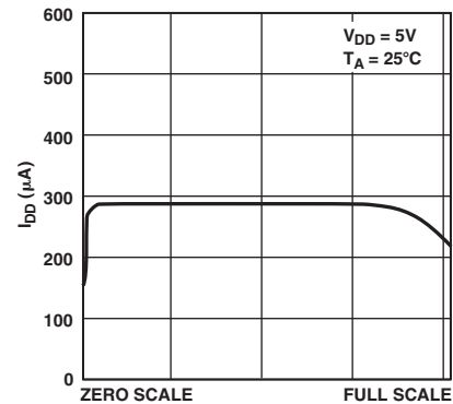
TPC 12. Supply Current vs. Code
