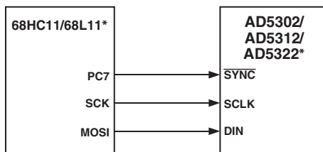
Figure 11. AD5302/AD5312/AD5322 to 68HC11/68L11 Interface
