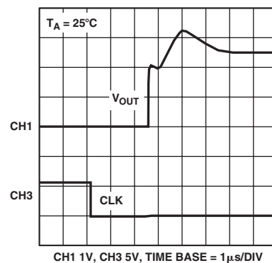
TPC 18. Existing Power-Down to Midscale
