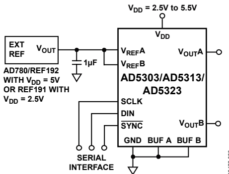
Figure 39. AD5303/AD5313/AD5323 Using External Reference
