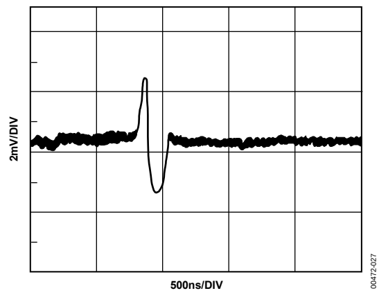
Figure 27. DAC-to-DAC Crosstalk
