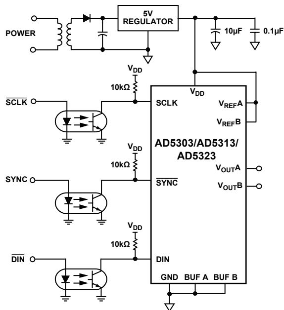
Figure 42. AD5303/AD5313/AD5323 in an Opto-Isolated Interface
