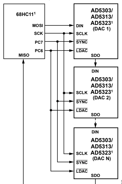
Figure 46. Daisy-Chain Mode
