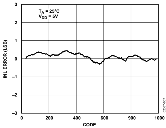
Figure 7. AD5317 INL
