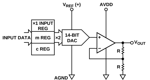
Figure 26. Single-Channel Architecture
