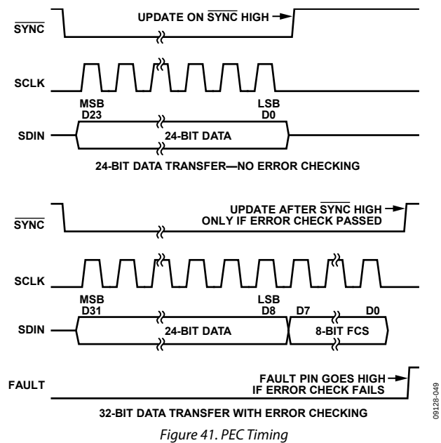
Figure 41. PEC Timing
