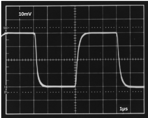
Figure 21. Unity-Gain Follower Small Signal Pulse Response
