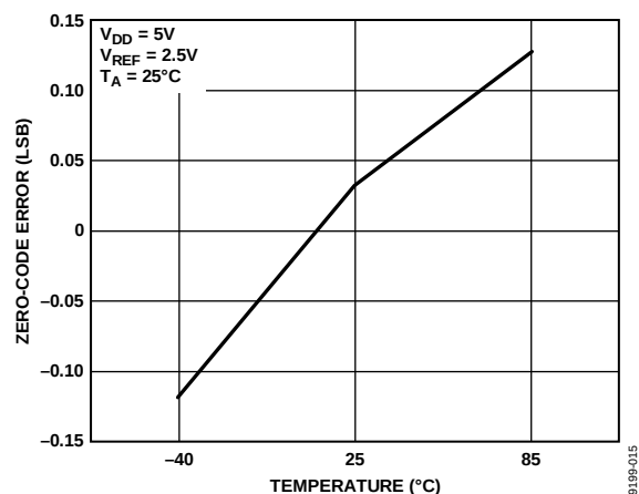
Figure 16. AD5512A/AD5542A Zero-Code Error vs. Temperature
