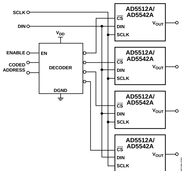
Figure 39. Addressing Multiple DACs
