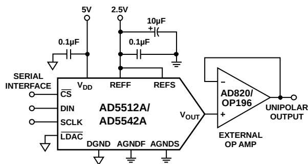
Figure 31. Unipolar Output
