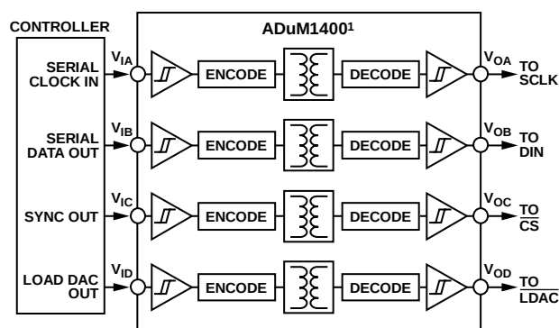
Figure 38. Isolated Interface
