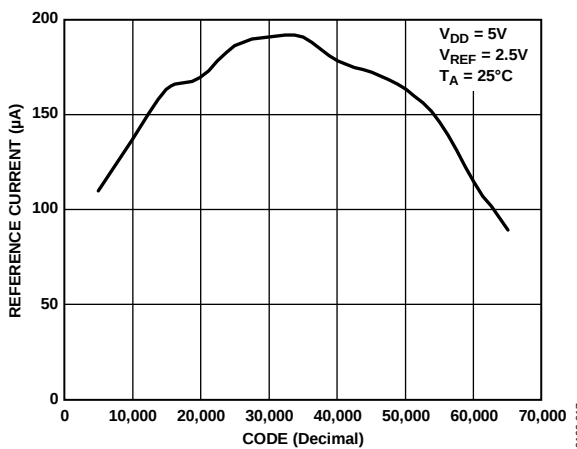
Figure 18. AD5512A/AD5542A Reference Current vs. Code
