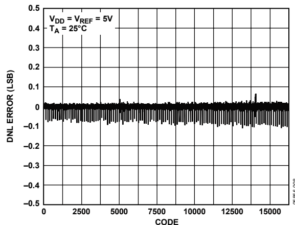
Figure 8. DNL AD5644R, External Reference
