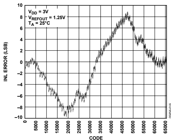
Figure 16. INL AD5664R-3, Internal Reference
