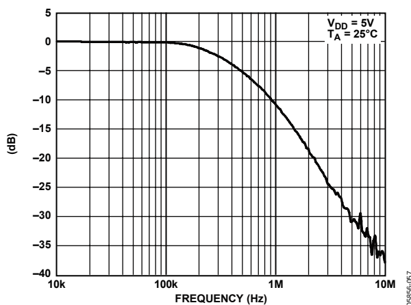
Figure 49. Multiplying Bandwidth
