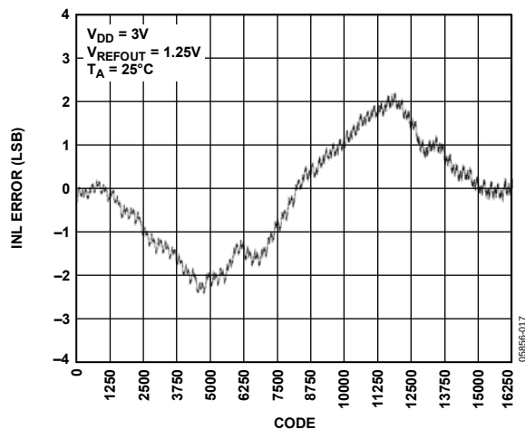
Figure 17. INL AD5644R-3, Internal Reference
