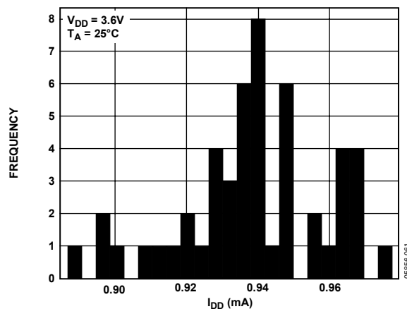
Figure 32. I_{DD} Histogram with Internal Reference, V_{REFOUT} = 1.25\text{V}
