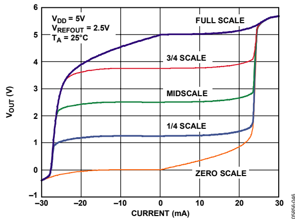
Figure 34. AD56x4R-5 Source and Sink Capability
