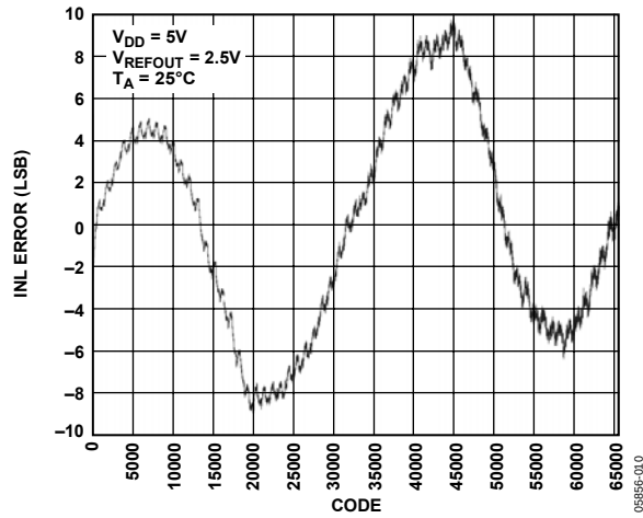
Figure 10. INL AD5664R-5, Internal Reference
