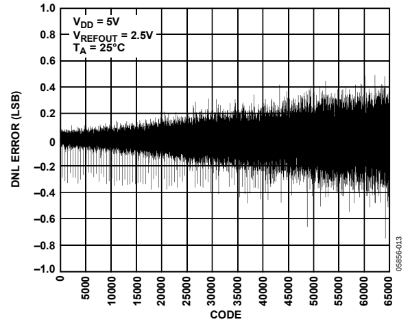
Figure 13. DNL AD5664R-5, Internal Reference
