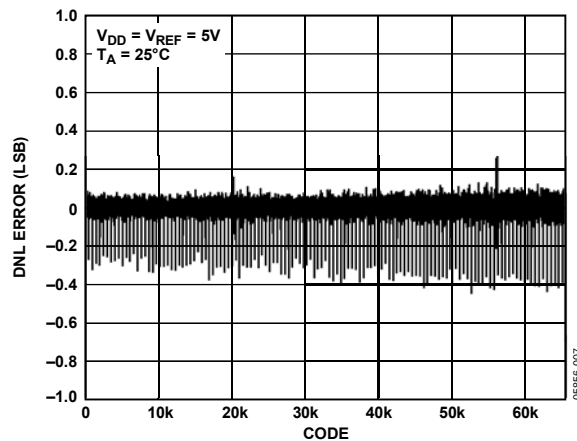
Figure 7. DNL AD5664R, External Reference
