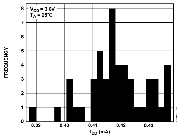
Figure 31. I_{DD} Histogram with External Reference, 3.6 V
