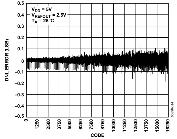
Figure 14. DNL AD5644R-5, Internal Reference
