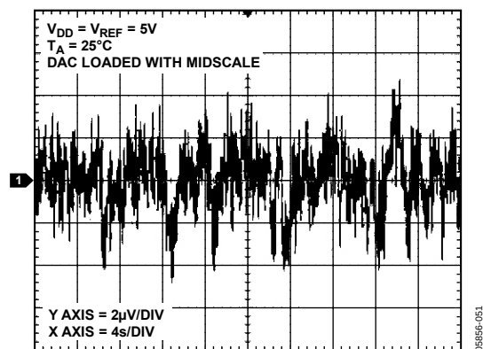
Figure 43. 0.1 Hz to 10 Hz Output Noise Plot, External Reference
