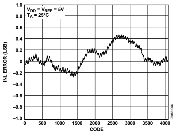
Figure 6. INL AD5624R, External Reference
