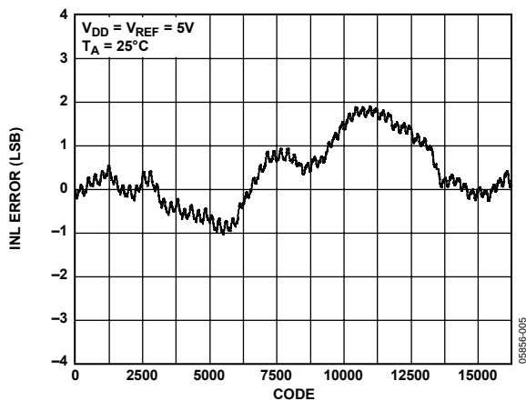
Figure 4. INL AD5664R, External Reference
