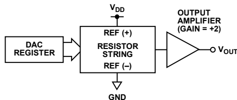
Figure 50. DAC Architecture
