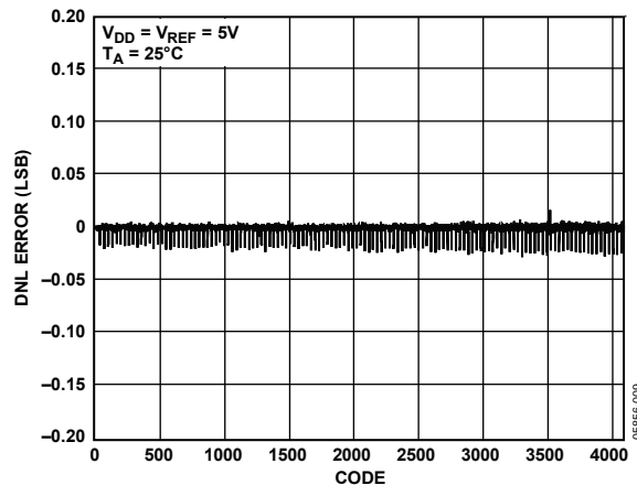
Figure 9. DNL AD5624R, External Reference
