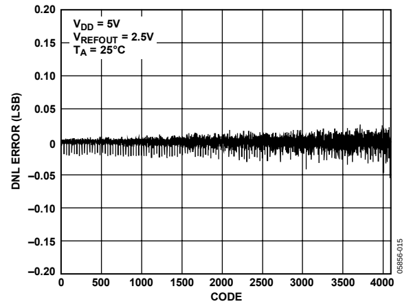
Figure 15. DNL AD5624R-5, Internal Reference
