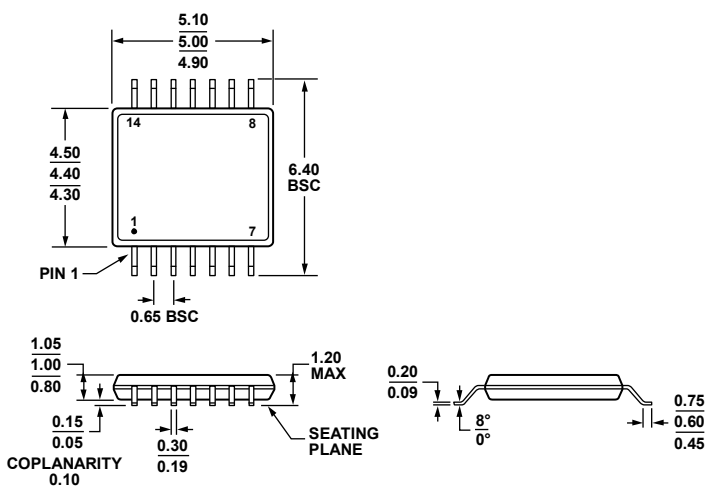
Figure 75. 14-Lead Thin Shrink Small Outline Package [TSSOP] (RU-14) Dimensions shown in millimeters
