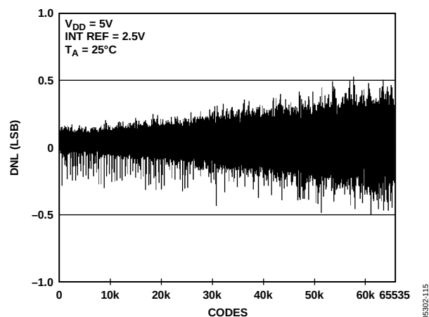
Figure 16. DNL AD5668-2/AD5668-3
