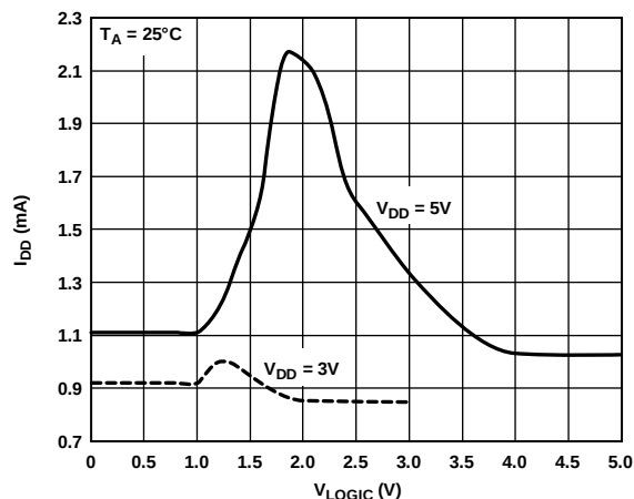
Figure 37. Supply Current vs. Logic Input Voltage
