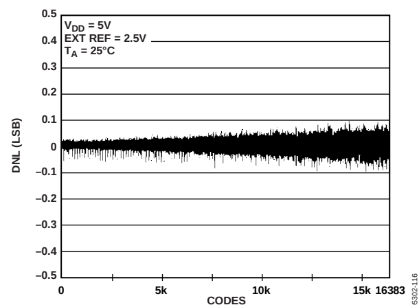
Figure 17. DNL AD5648-2
