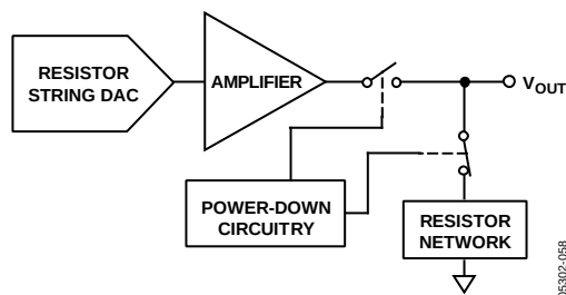
Figure 61. Output Stage During Power-Down
