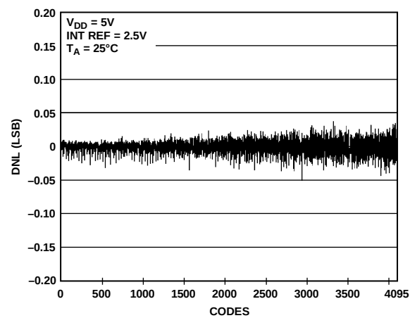
Figure 18. DNL AD5628-2
