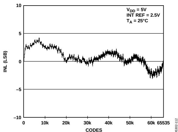
Figure 13. INL AD5668-2/AD5668-3
