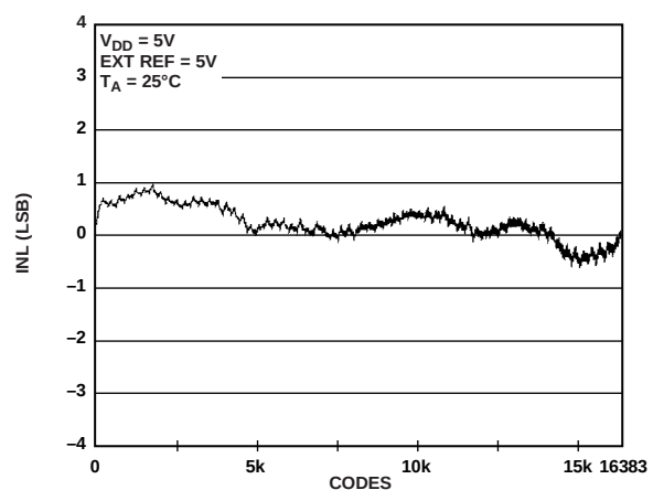
Figure 14. INL AD5648-2
