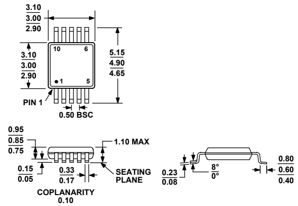
Figure 64. 10-Lead Mini Small Outline Package [MSOP] (RM-10) Dimensions shown in millimeters
