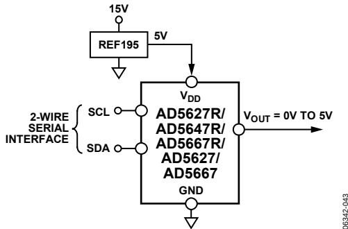
Figure 67. REF195 as Power Supply to the AD56x7R/AD56x7
